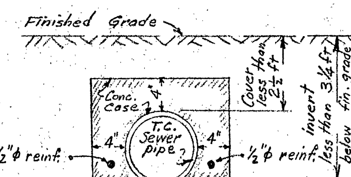
Typical Section - Concrete Case
