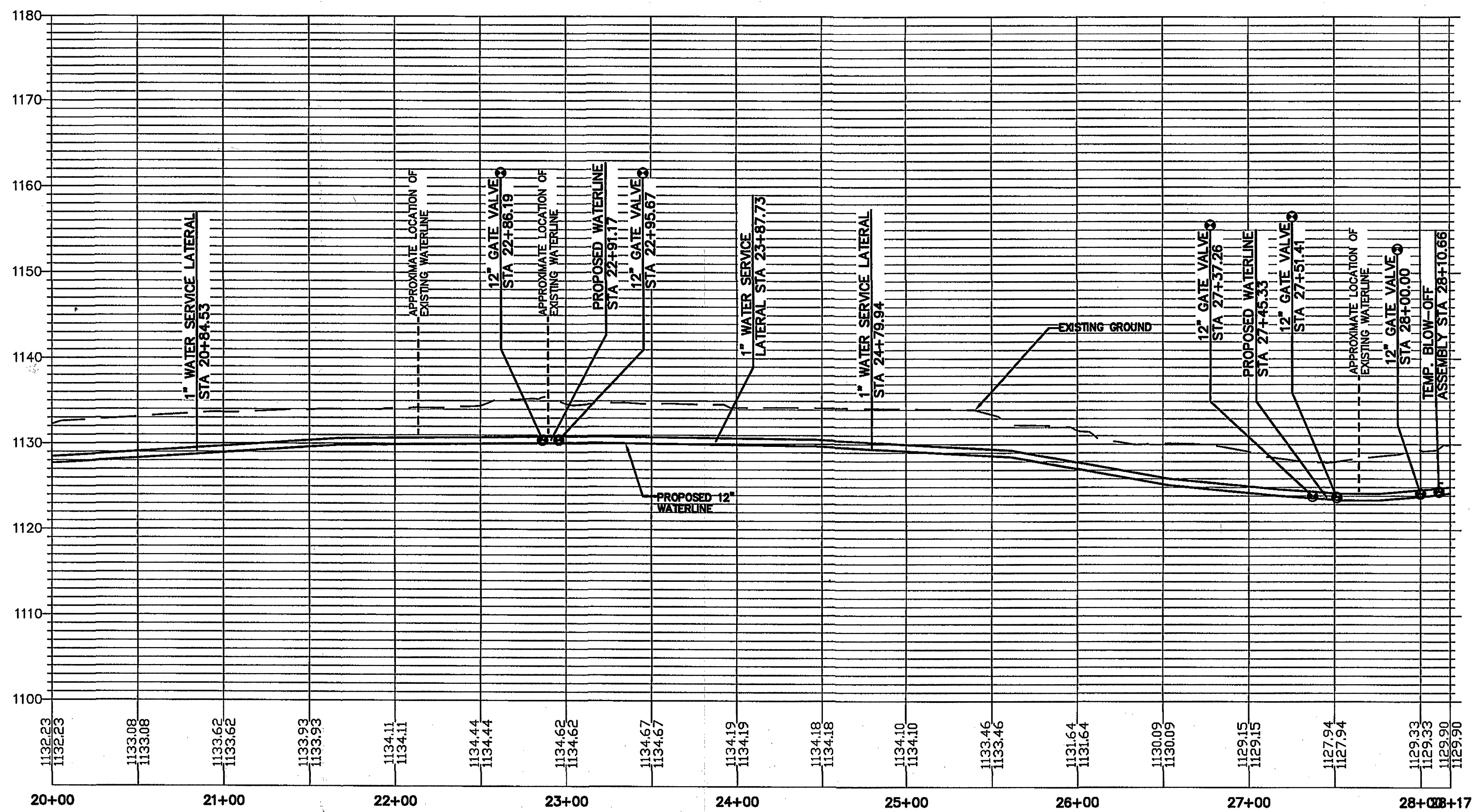
RUTROUGH RD. STA 20+00.00 TO STA 28+17.38 PROFILE
