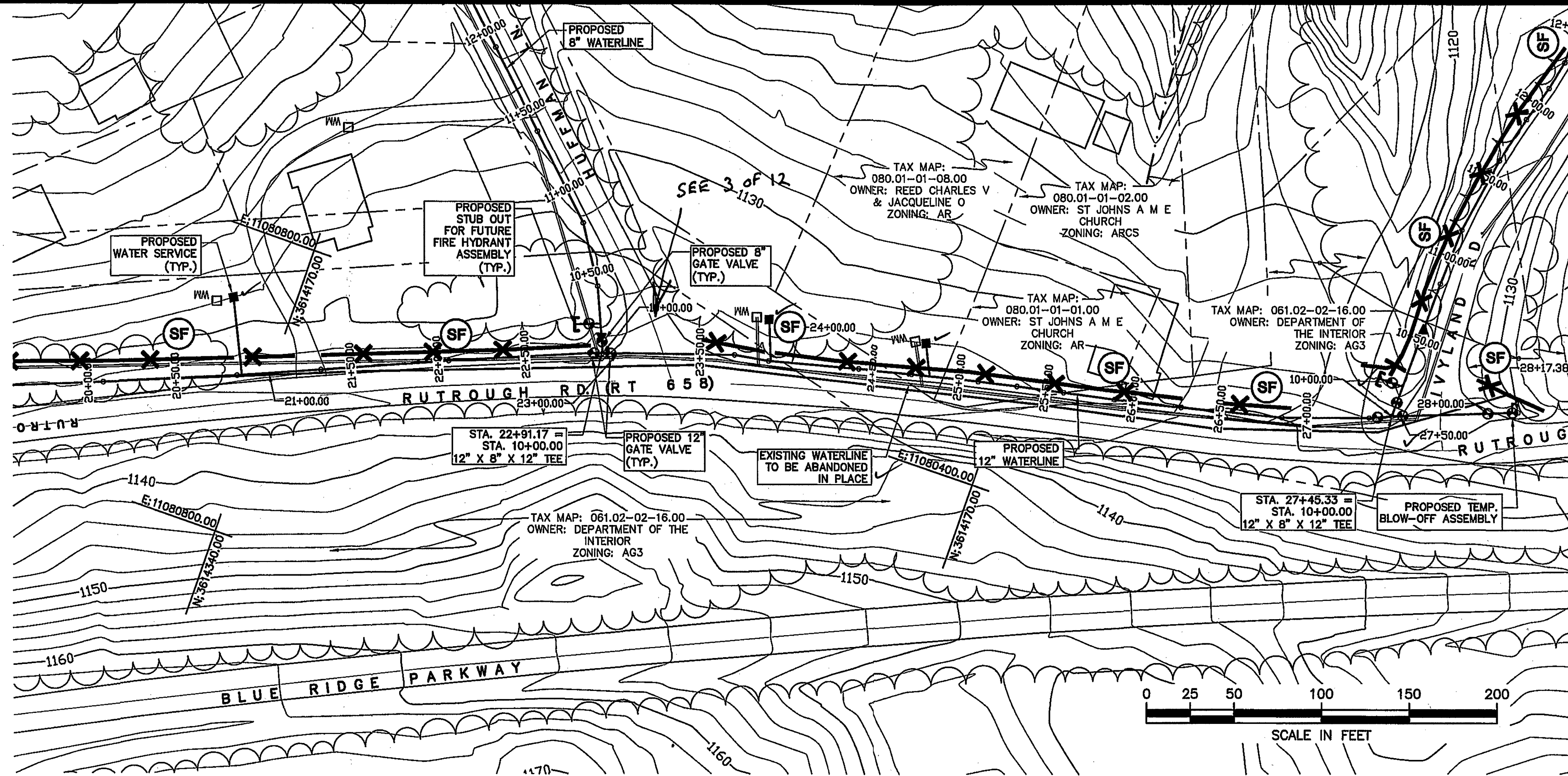
RUTROUGH RD. STA 20+00.00 TO STA 28+17.38 PLAN
