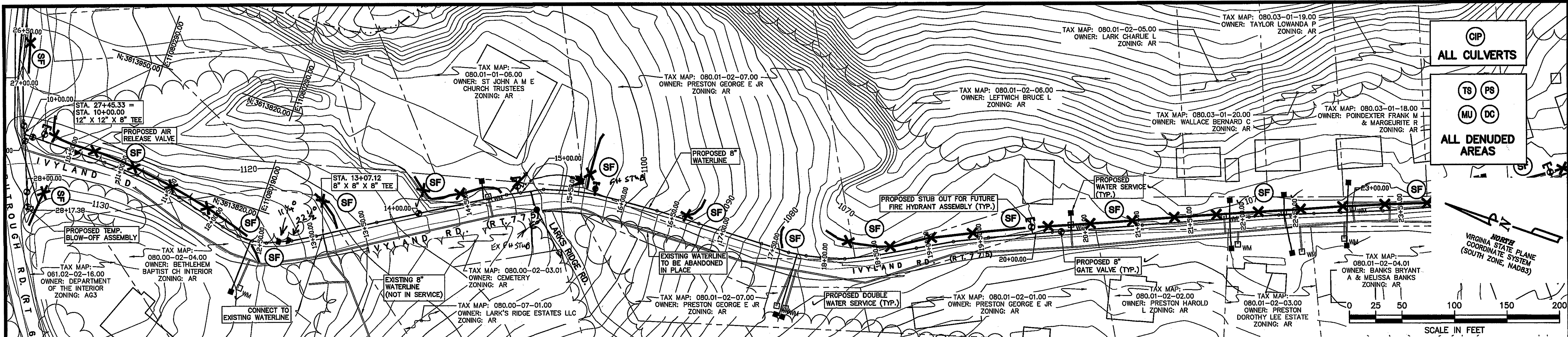
IVYLAND RD. STA 10+00.00 TO STA 23+00.00 PLAN SCALE: 1"=50'
