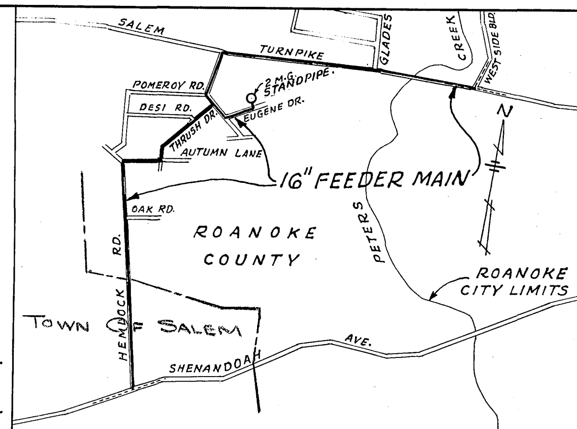
LOCATION PLAN SCALE: 1" = 1200'
