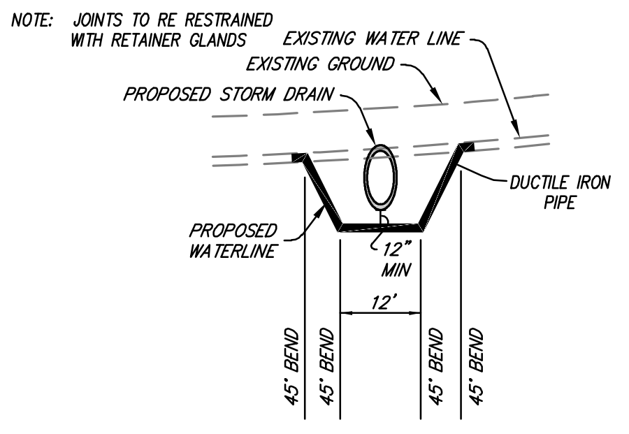
NOTE: WATERLINE RELOCATION SHALL PROVIDE A MINIMUM COVER OF 30 INCHES OVER THE WATERLINE. COORDINATE ALL WORK WITH THE WESTERN VIRGINIA WATER AUTHORITY.
