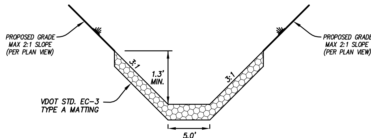
SEE VDOT STANDARDS FOR VDOT STD. EC-3 TYPE A SPECIFICATIONS
