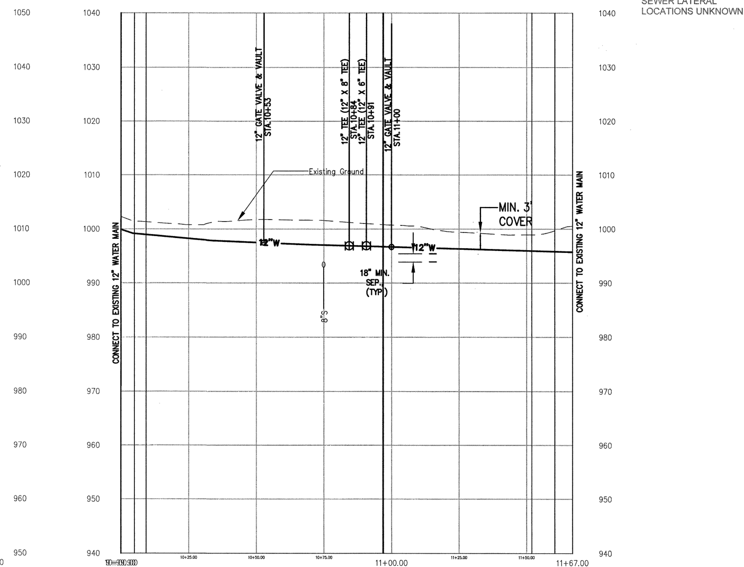
12" WATER MAIN IN GRANDIN RD.
