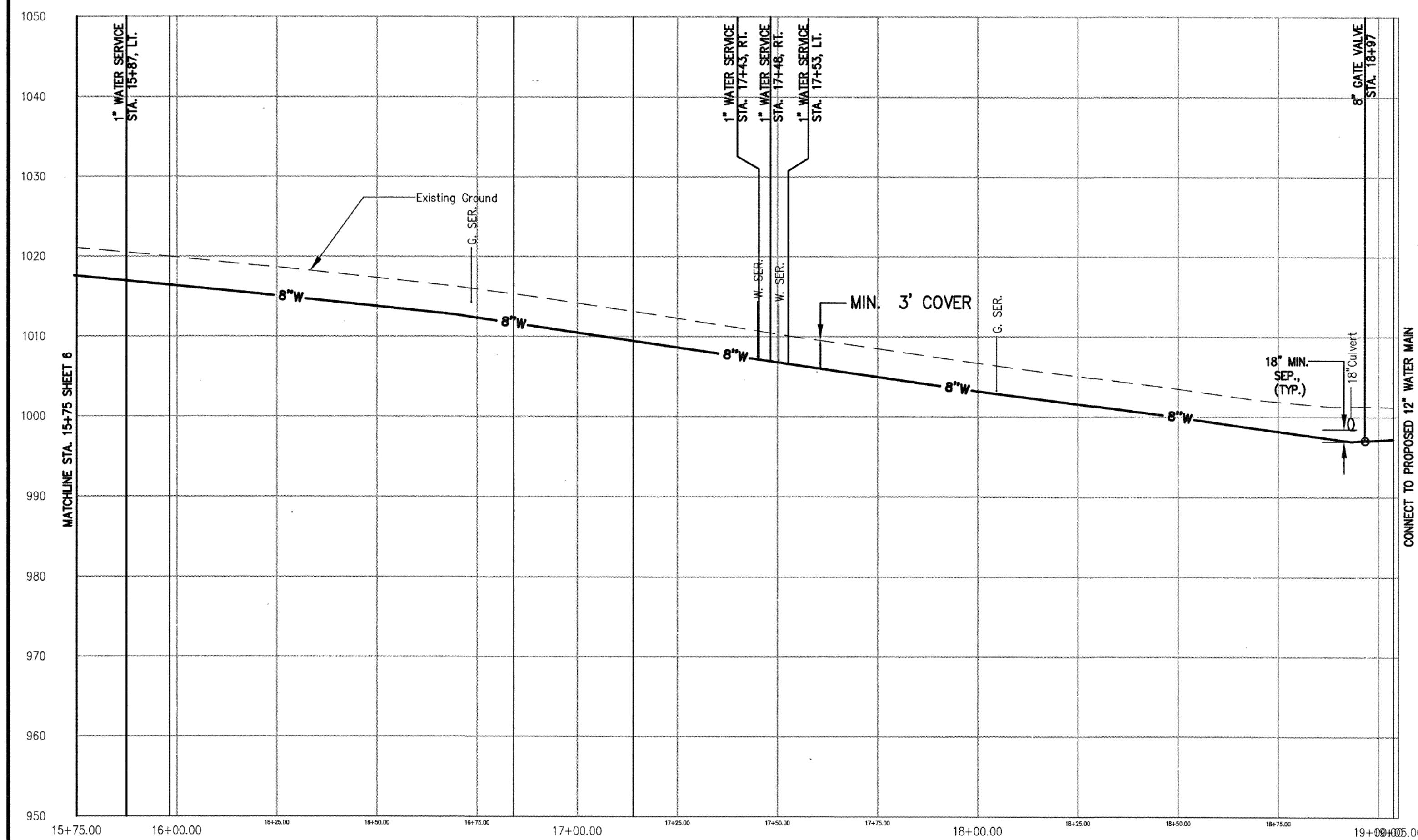
8" WATER MAIN IN DOVER DR.
