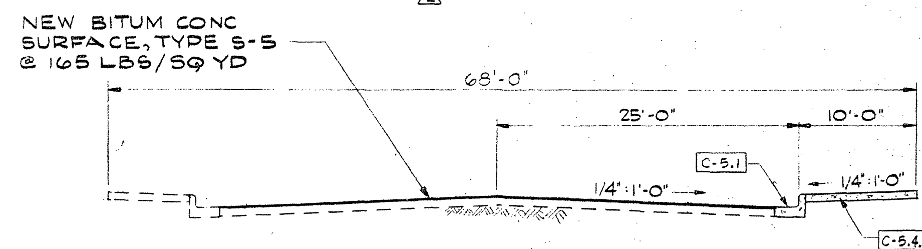
SECTION 2.3 NO SCALE
