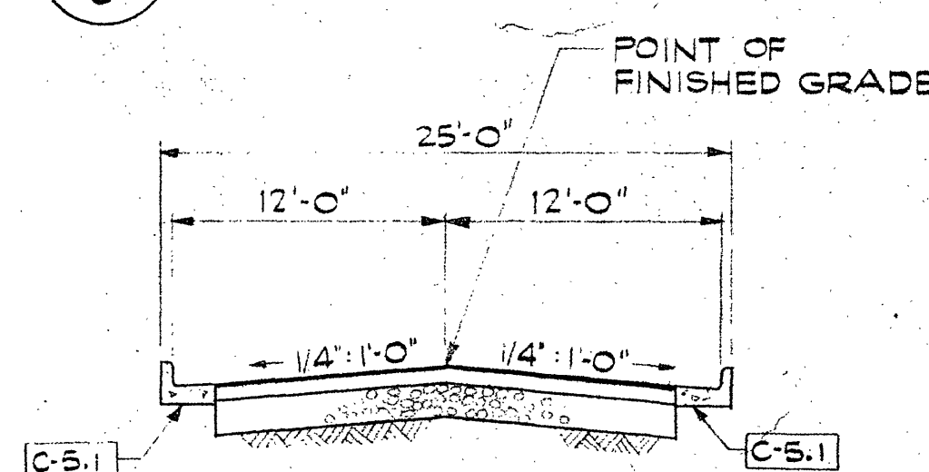
SECTION 2.7 NO SCALE
