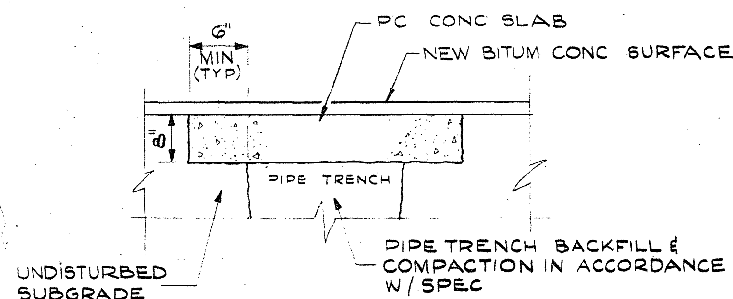
PAVEMENT REPLACEMENT DETAIL NO SCALE
