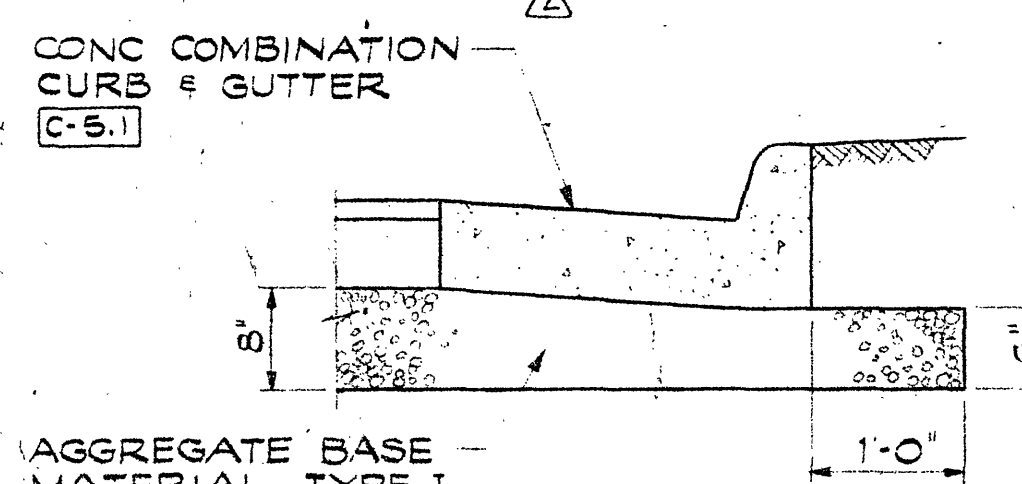
DETAIL 2.9 NO SCALE
