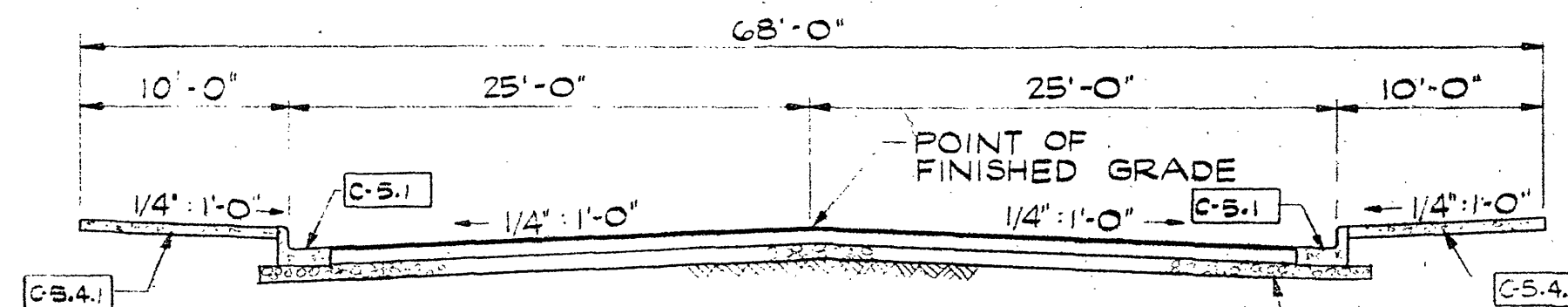
SECTION 2.4 NO SCALE
