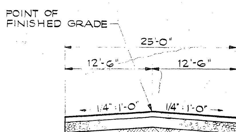
SECTION 2.6 NO SCALE
