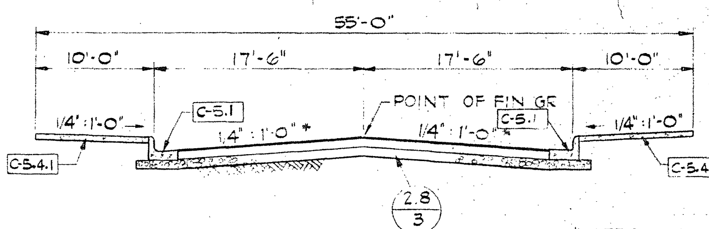
SECTION 2.5 NO SCALE
