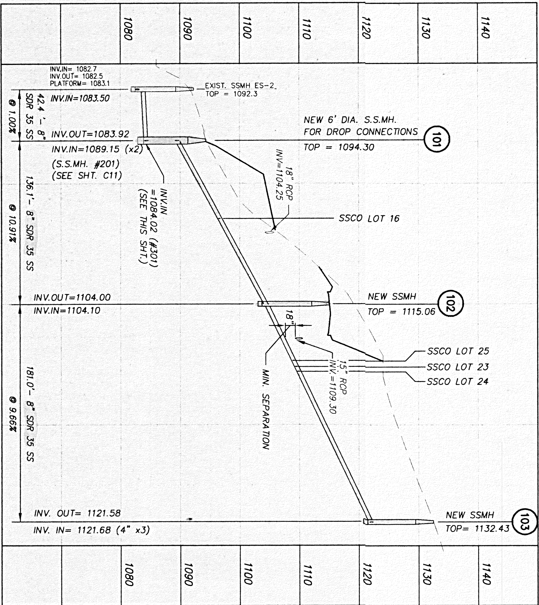
PROFILE: SANITARY SEWER 101 - 103 SCALES: 1" = 50' HORIZ. 1" = 10' VERT.
