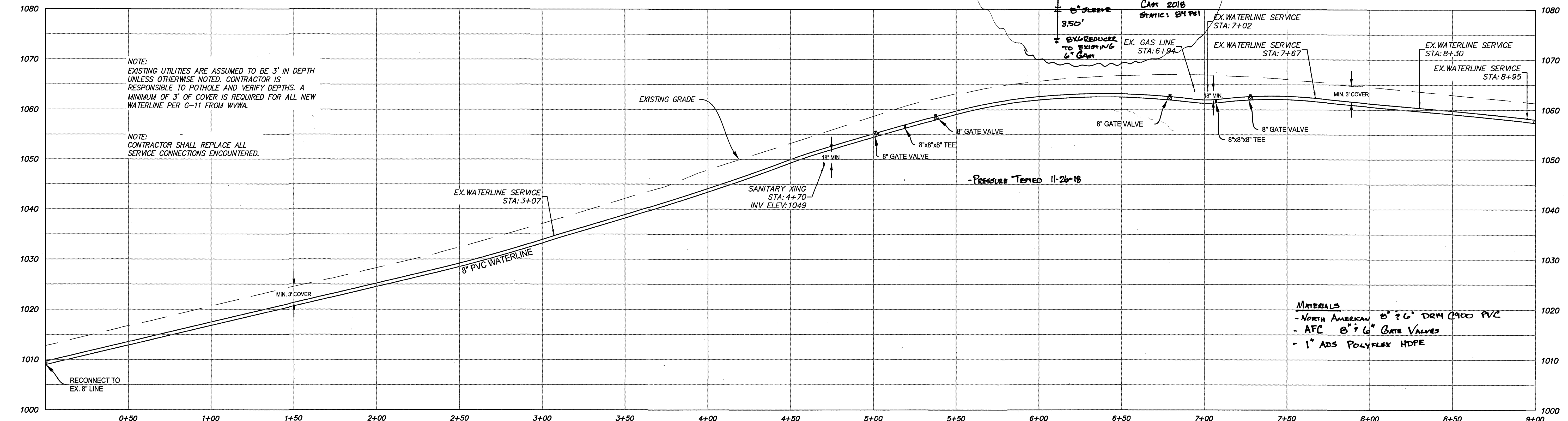
EDGEWOOD STREET S.W. 0+00 - 9+00 PROFILE 1" = 30' Horizontal 1" = 10' Vertical
