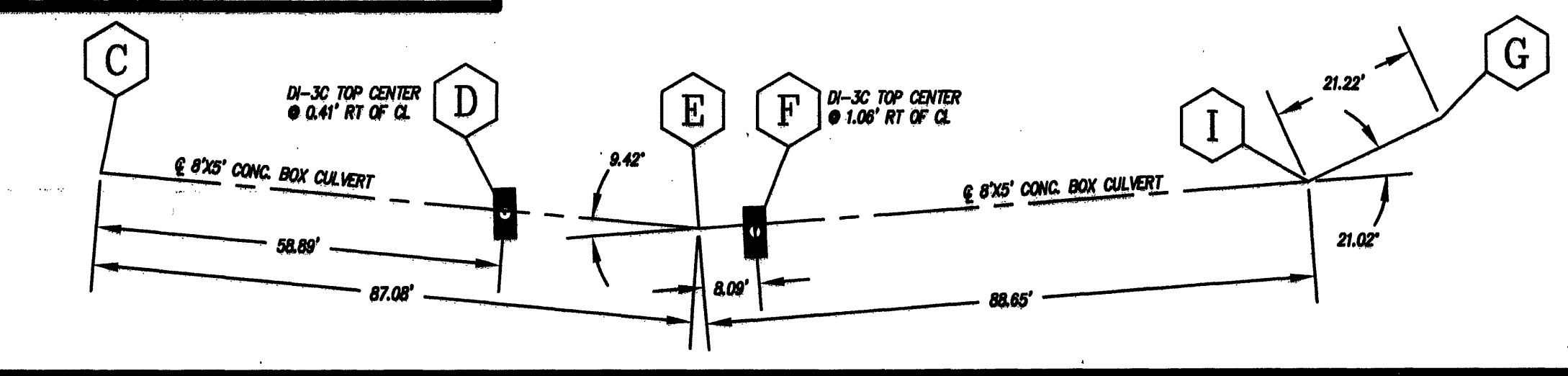
BOX CULVERT DIMENSIONS SCALE: 1" = 20'
