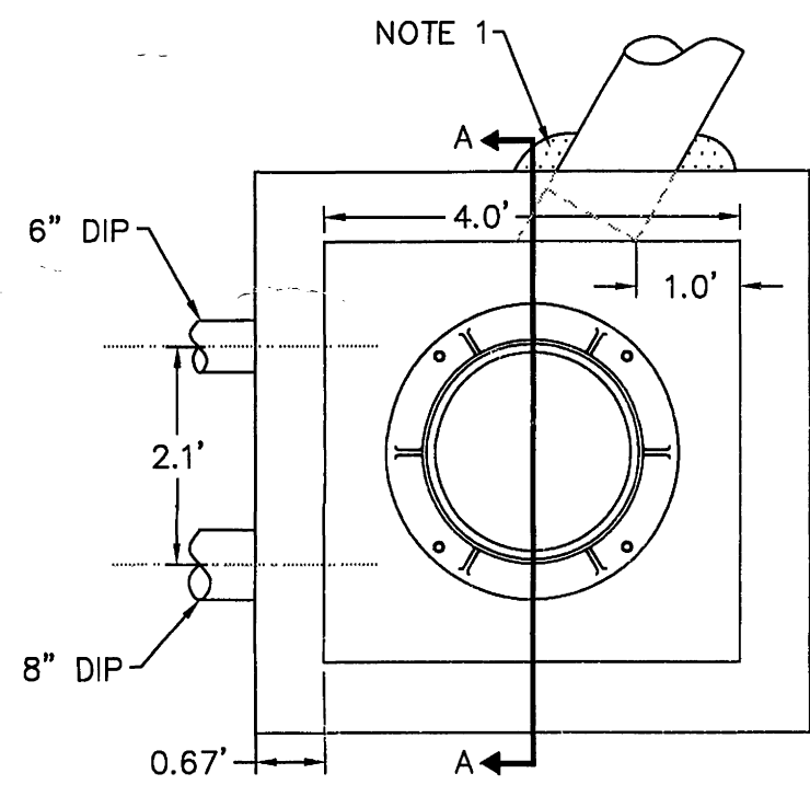
OUTLET STRUCTURE PRECAST JUNCTION BOX PER SPECIFICATION SECTION 02533 SCALE: 1"=2'
