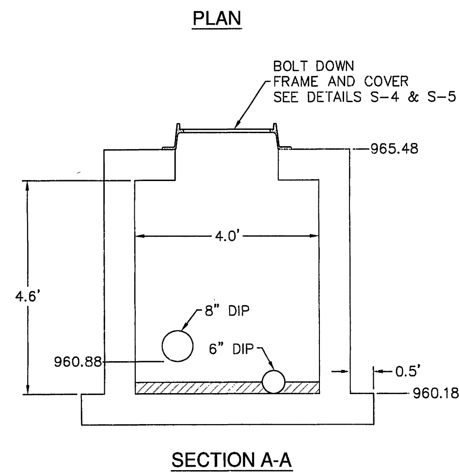
INLET STRUCTURE PRECAST JUNCTION BOX PER SPECIFICATION SECTION 02533 SCALE: 1"=2'
