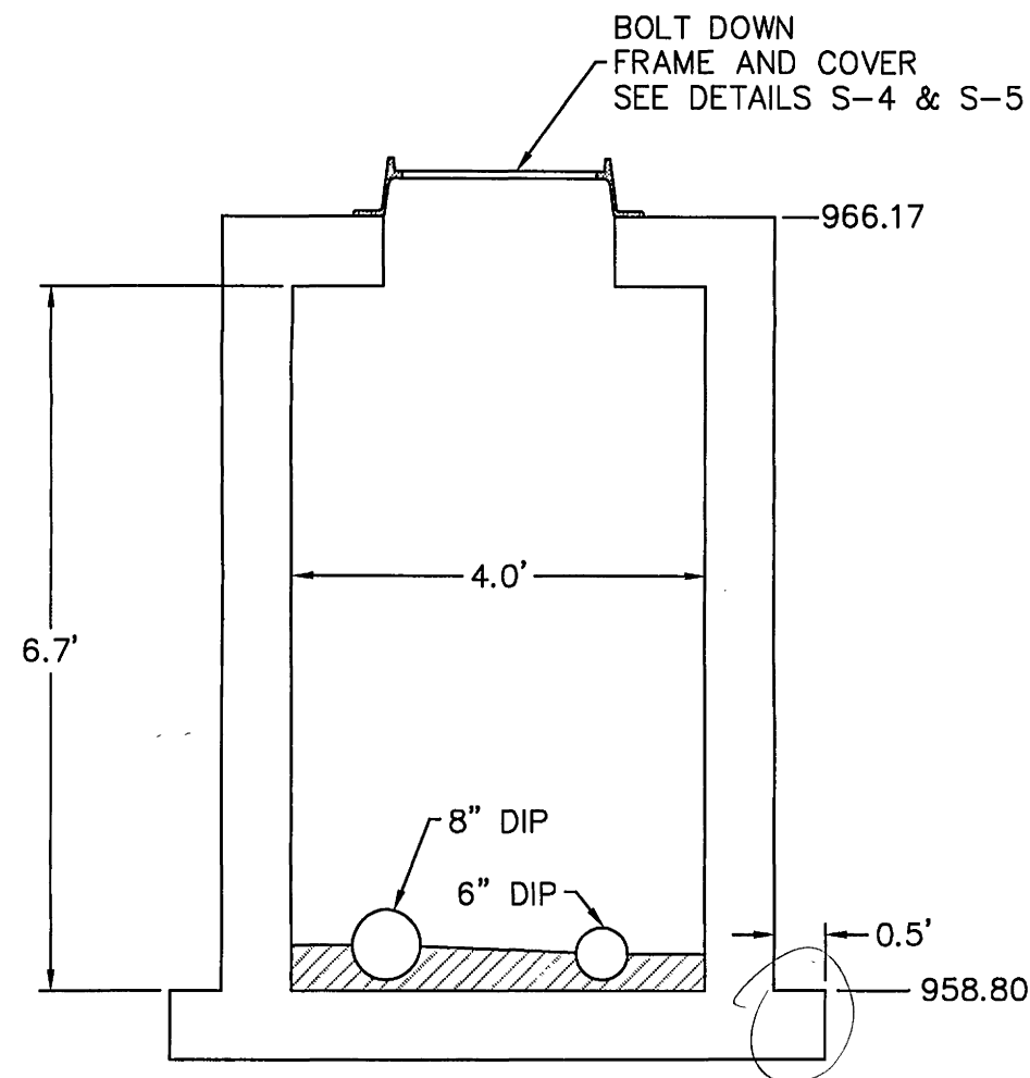
OUTLET STRUCTURE PRECAST JUNCTION BOX PER SPECIFICATION SECTION 02533 SCALE: 1"=2'
