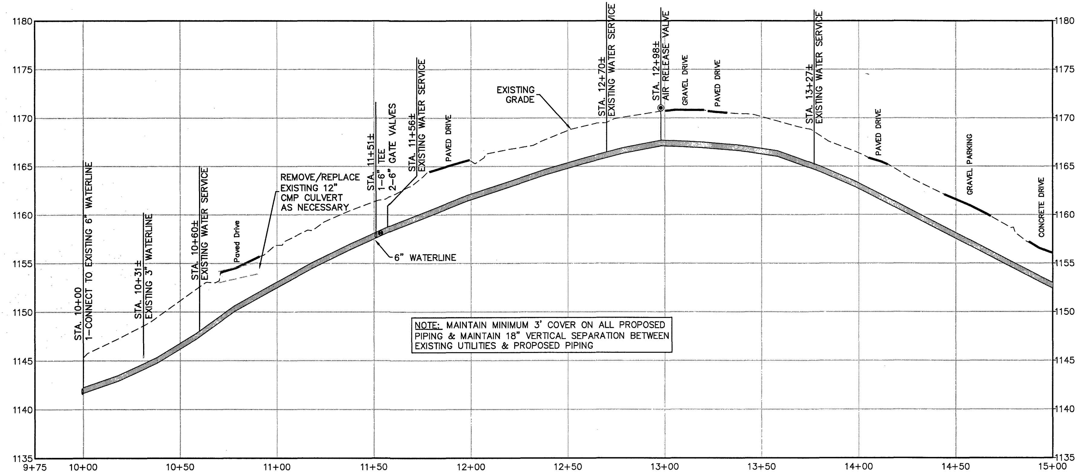
LINE B PROFILE SCALE: H: 1"=30' V: 1"=6'
