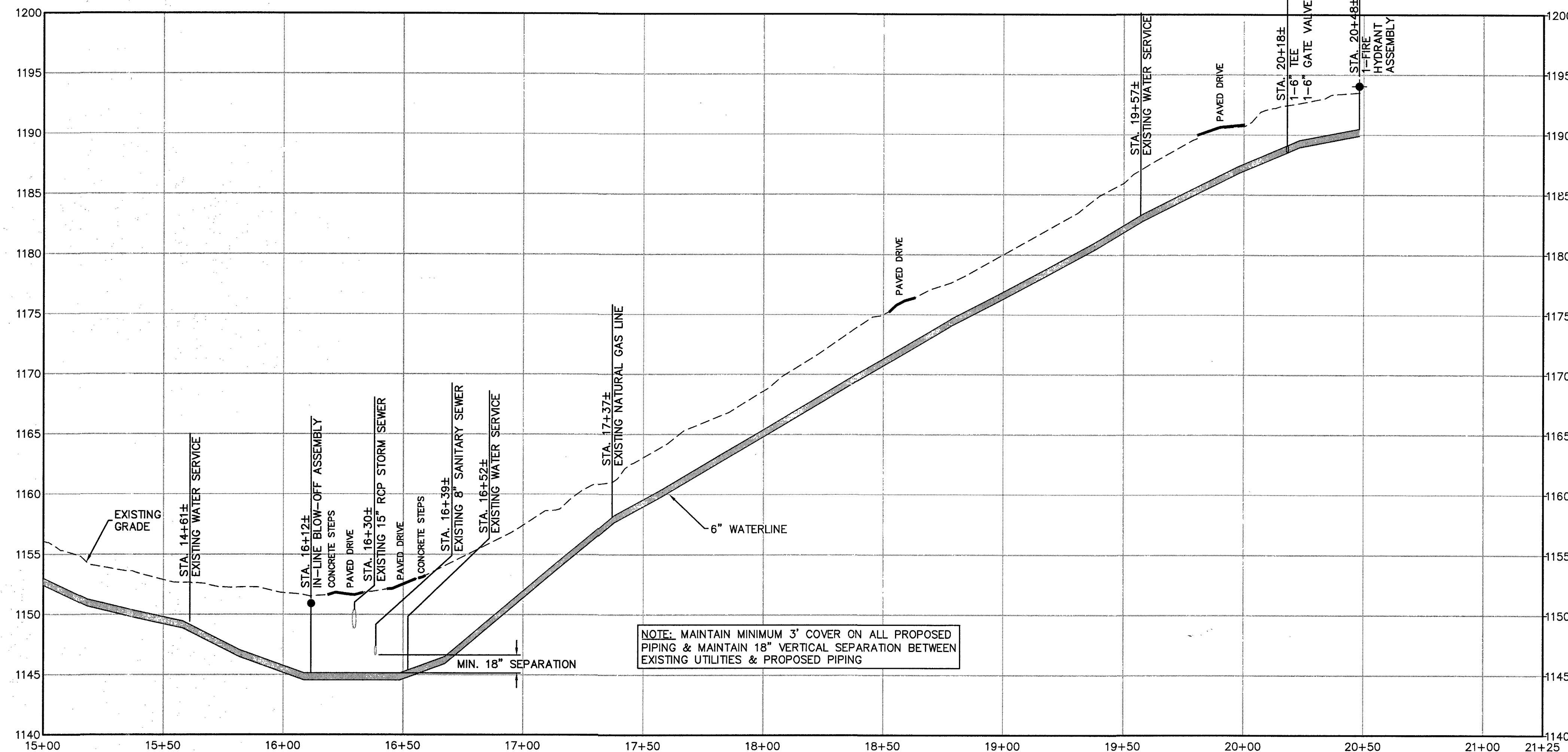
LINE B PROFILE SCALE: H: 1"=30' V: 1"=6'
