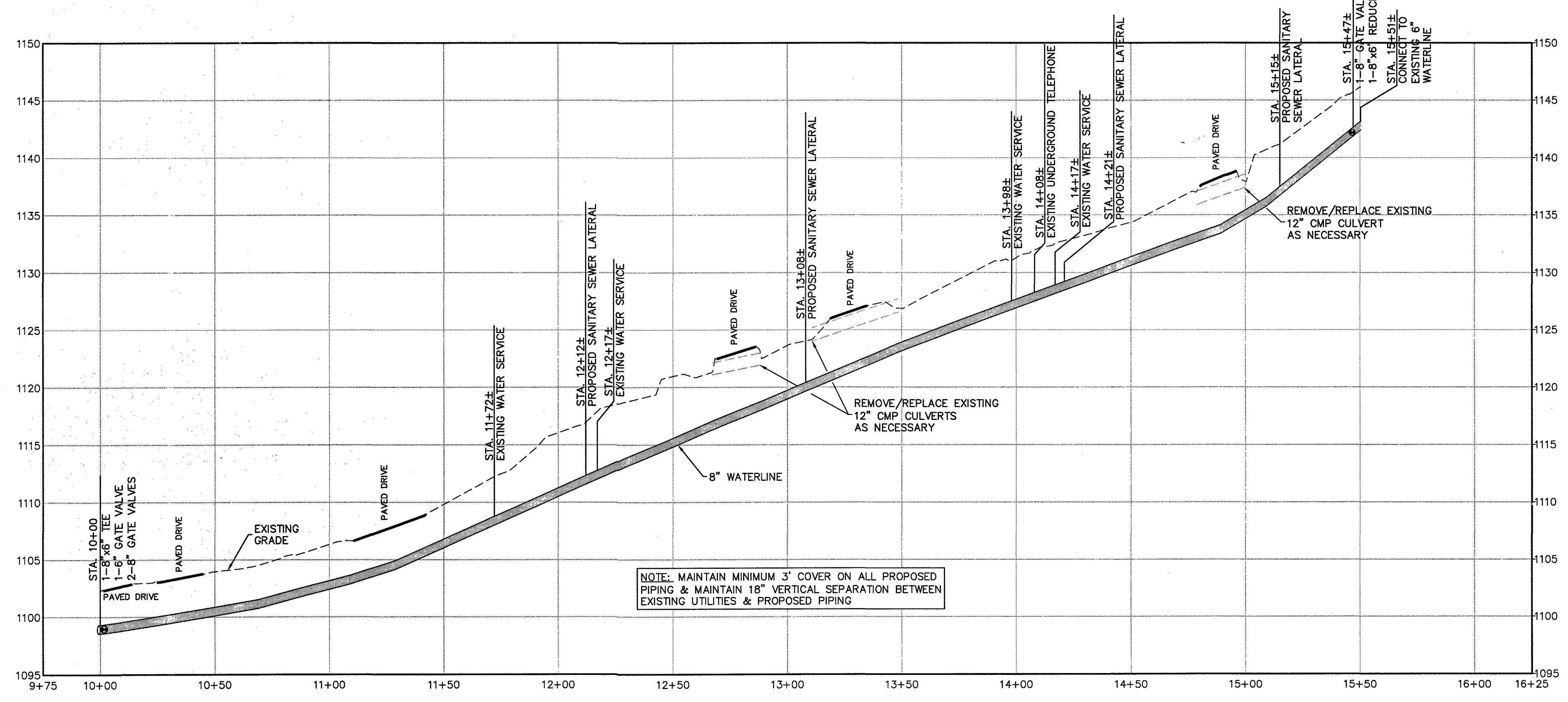
LINE D PROFILE SCALE: H: 1"=30' V: 1"=6'
