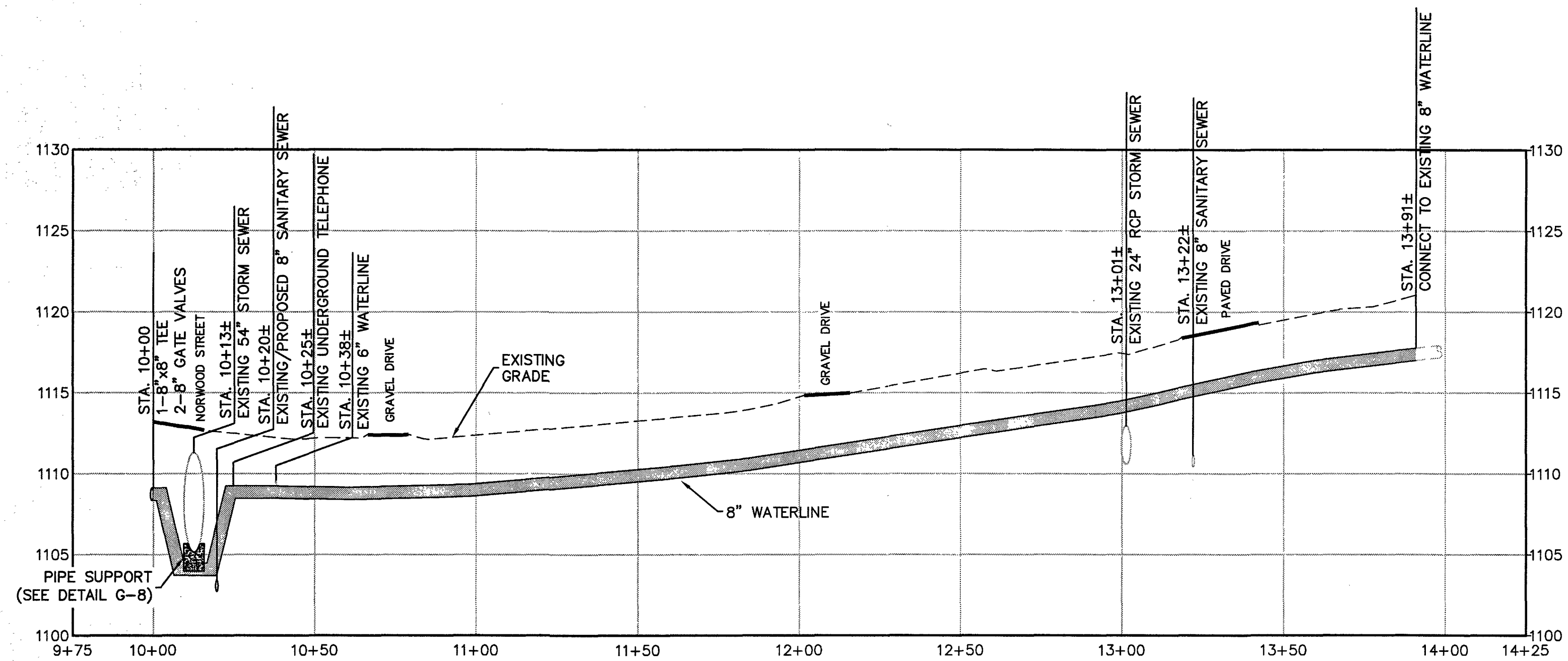
LINE G PROFILE SCALE: H: 1"=30' V: 1"=6'
