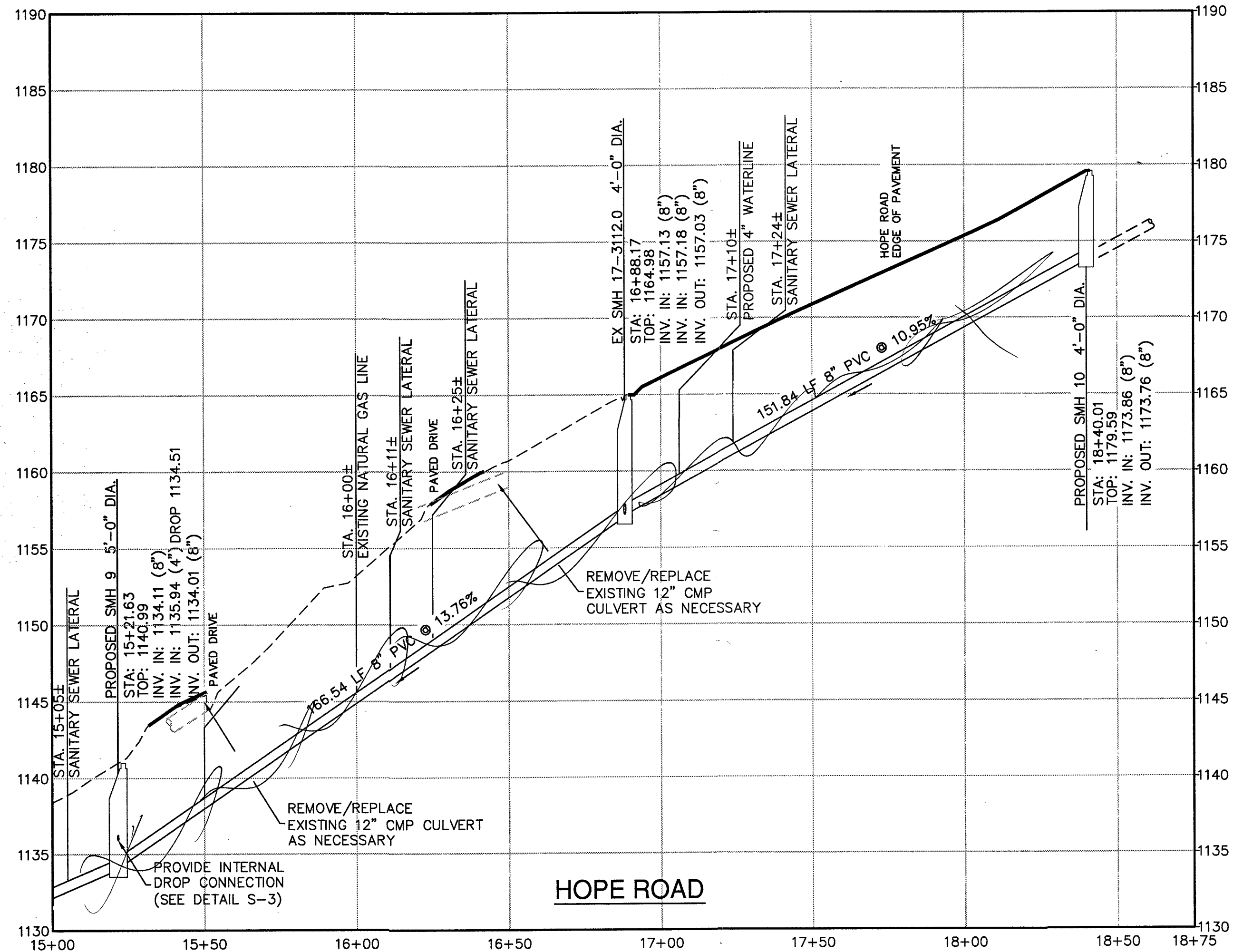
SEWER PROFILE SCALE: H: 1"=30', V: 1"=6'
