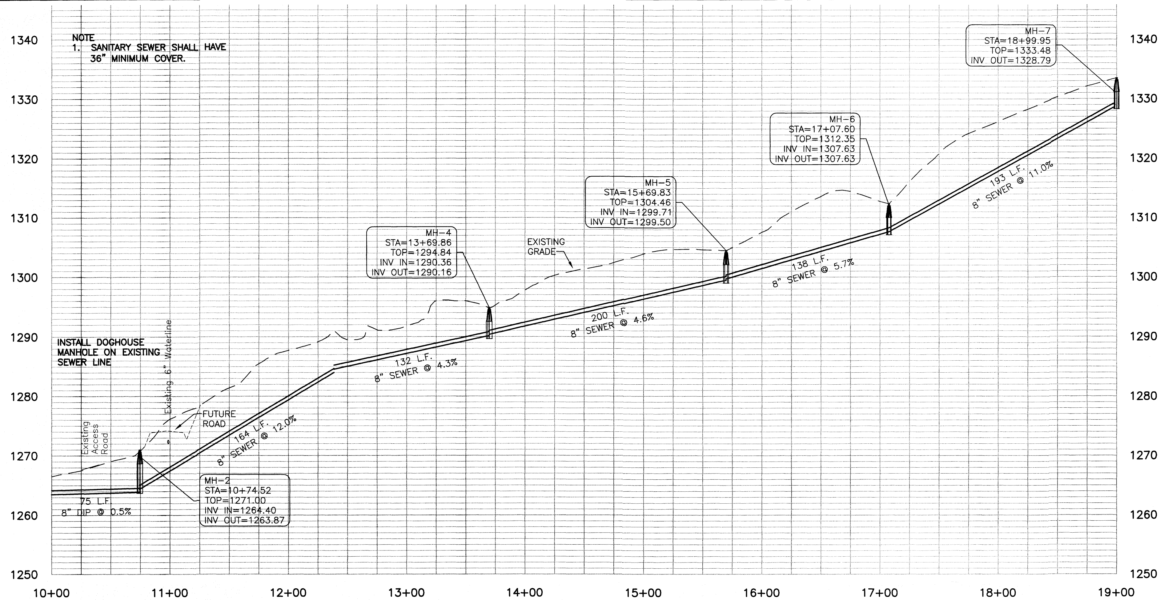
GRAVITY SEWER PROFILE SCALE: 1"=50'H, 1"=10'V
