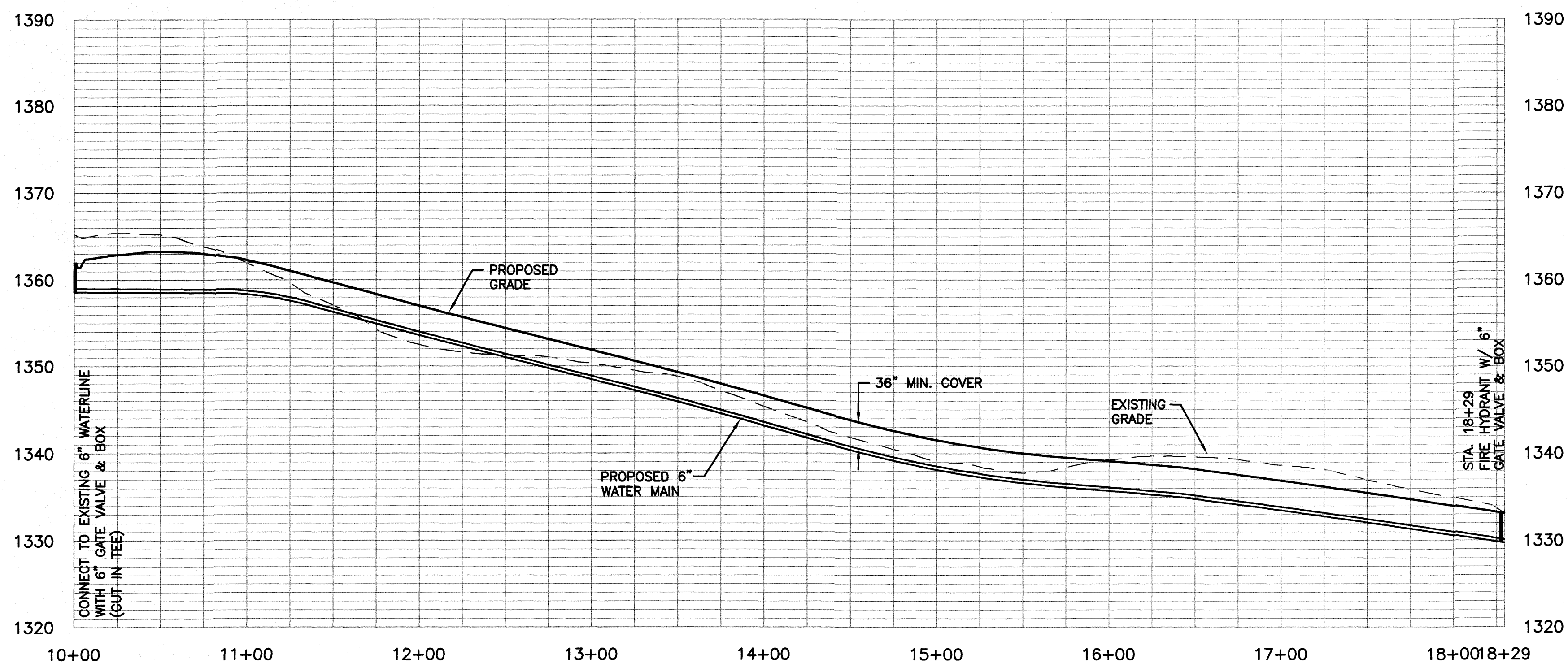
WATERLINE PROFILE SCALE: 1"=50'H, 1"=10'V
