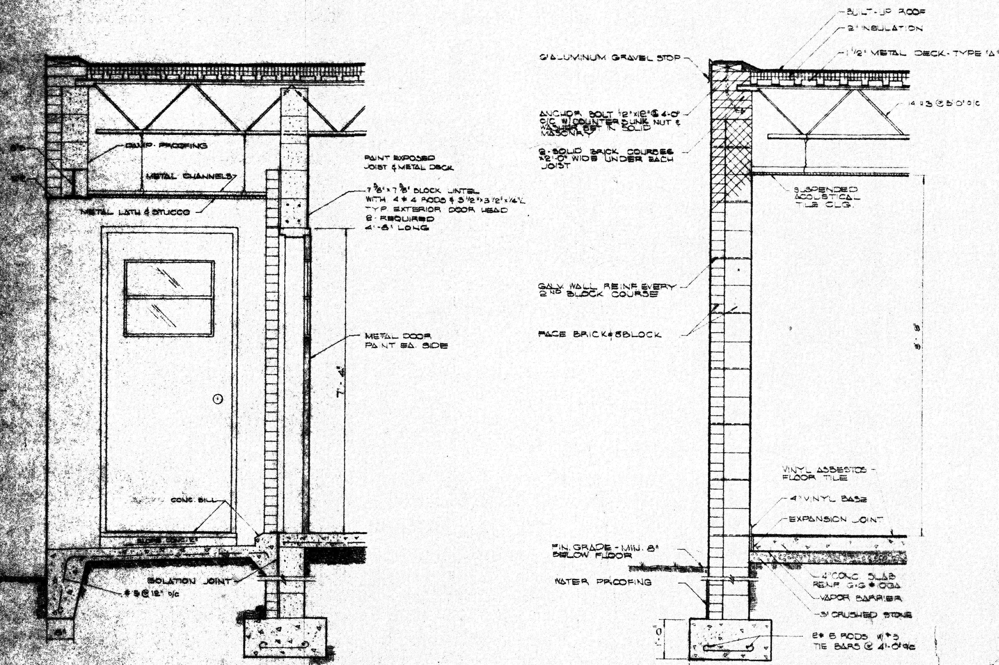
TYP. WALL SECTION SCALE: 3/4" = 1'-0"
