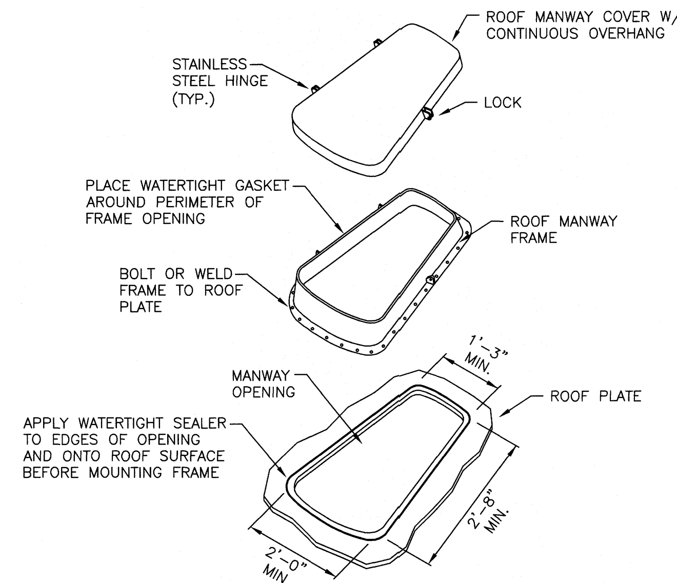
ROOF MANWAY DETAIL N.T.S.
