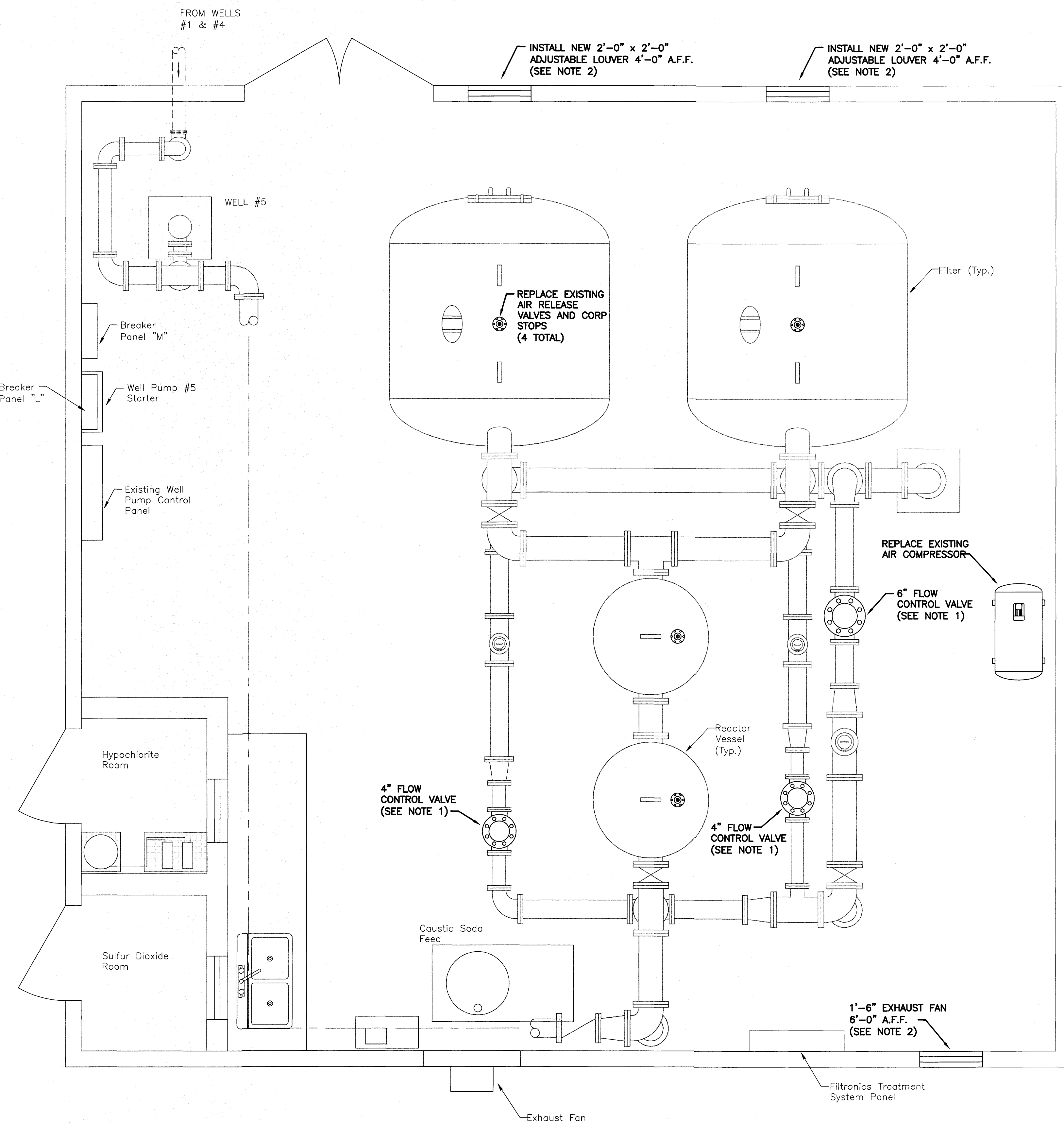
PLAN 1/2"=1'-0"
