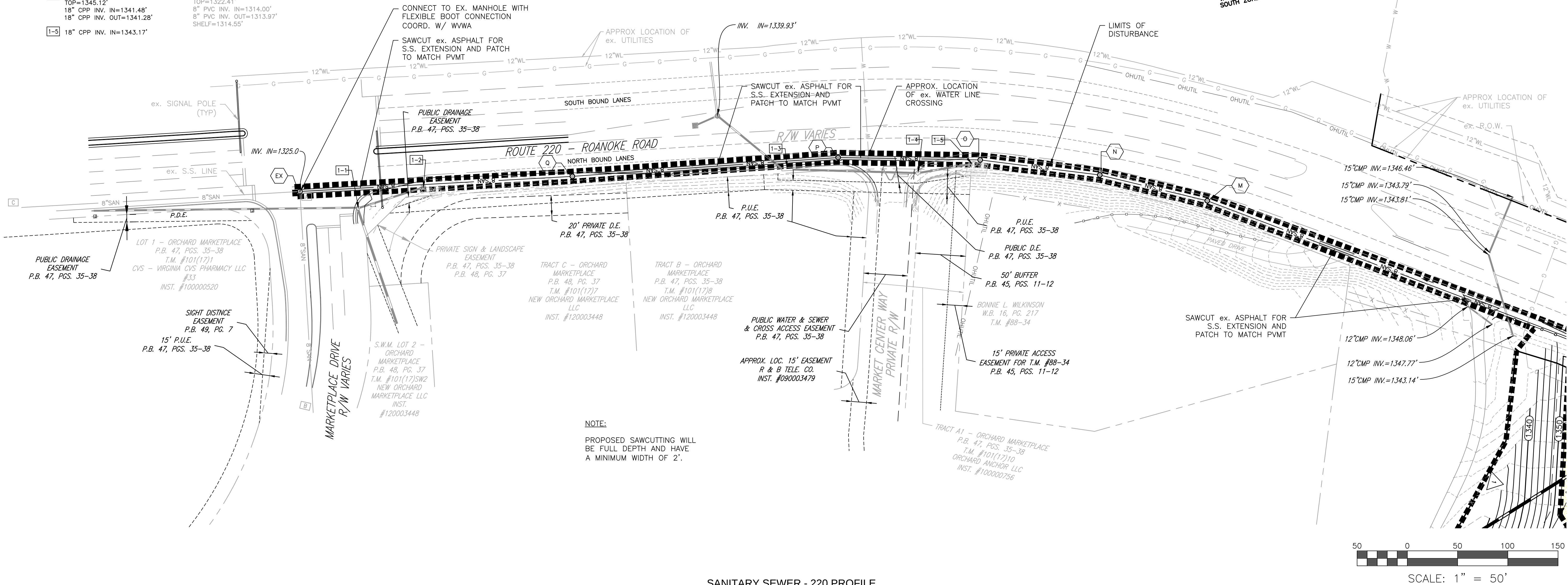
SANITARY SEWER - 220 PROFILE
