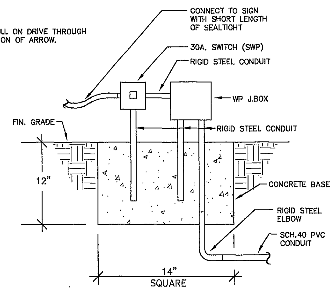
6 SWITCH & J.BOX MOUNTING DETAIL N.T.S.
