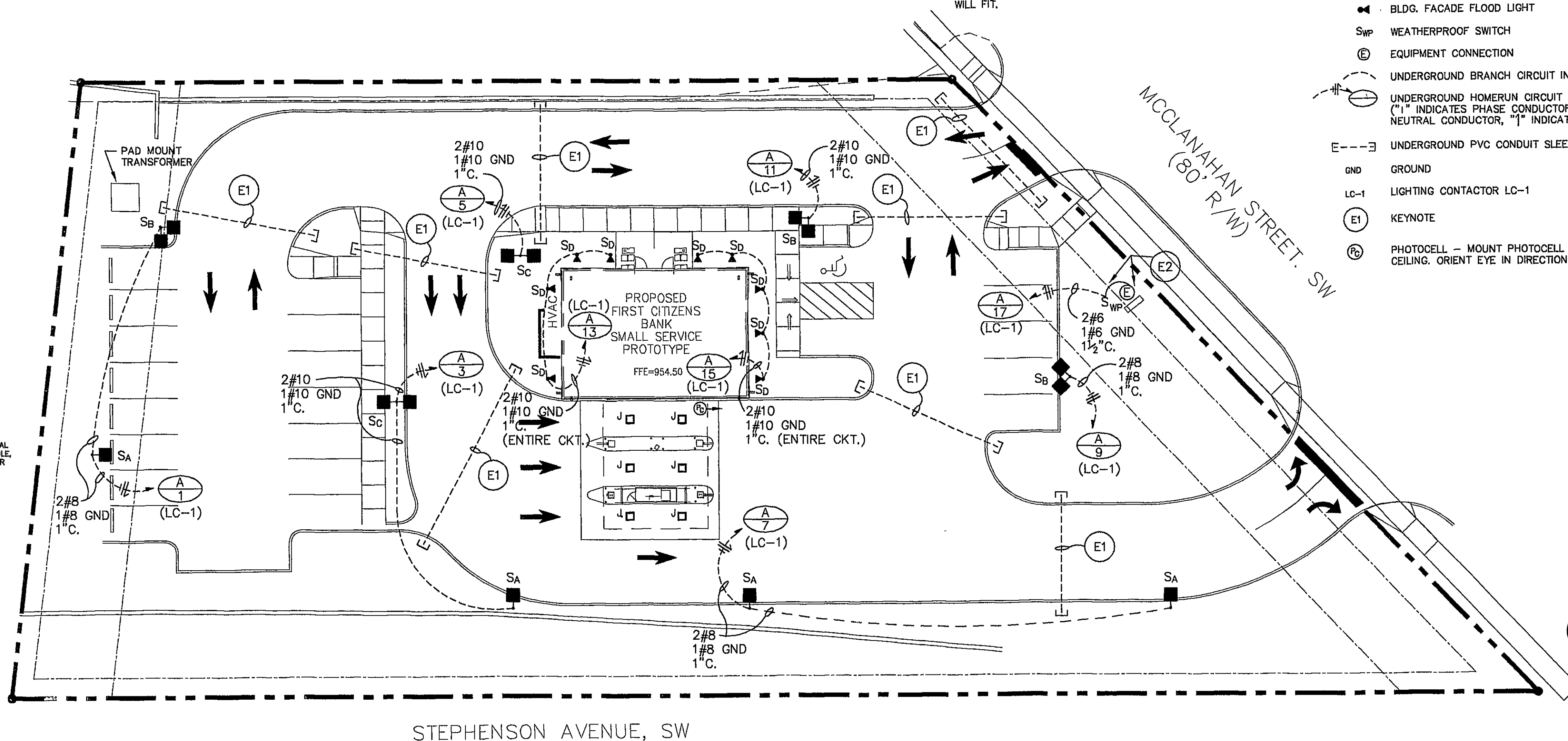
1 SITE LIGHTING PLAN SCALE: 1"=20'-0"
