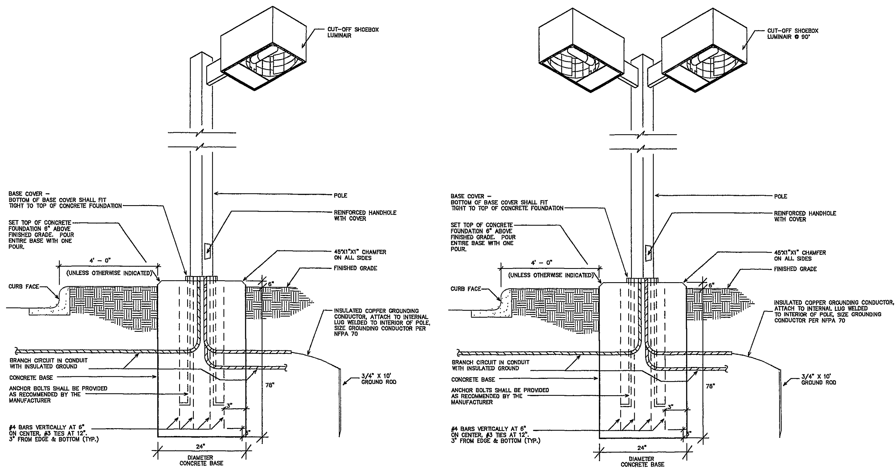
2 FIXTURE TYPE "SA" BASE DETAIL SL1 N.T.S.
