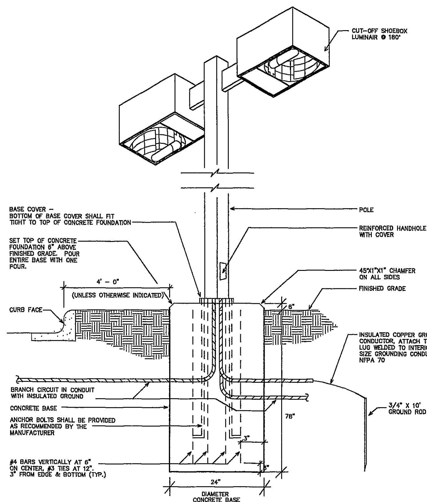
4 FIXTURE TYPE "SC" BASE DETAIL SL1 N.T.S.
