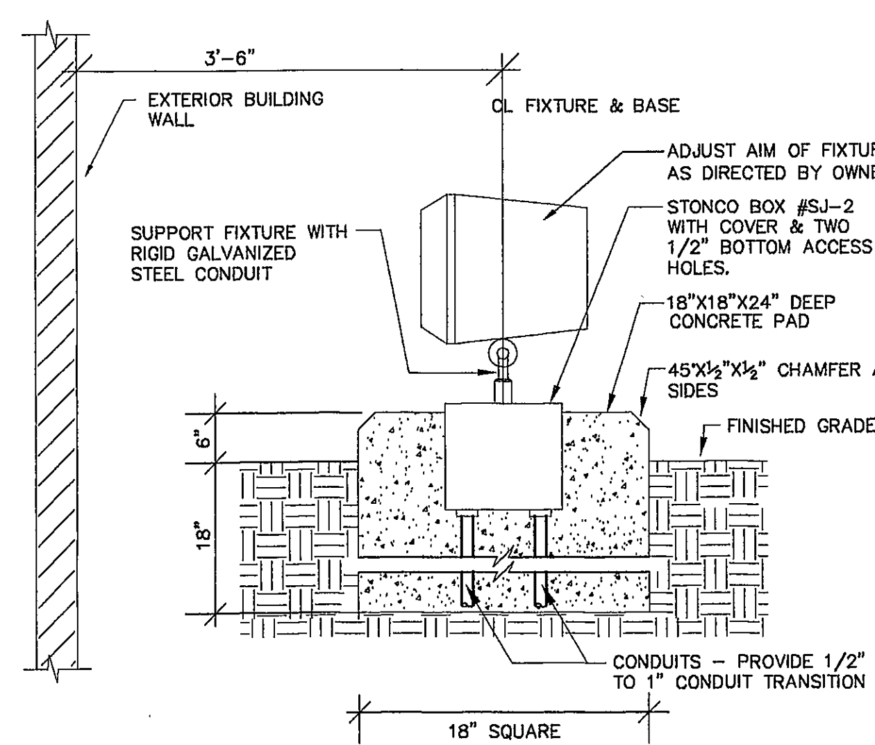
5 FIXTURE TYPE "SD" MOUNTING DETAIL N.T.S.
