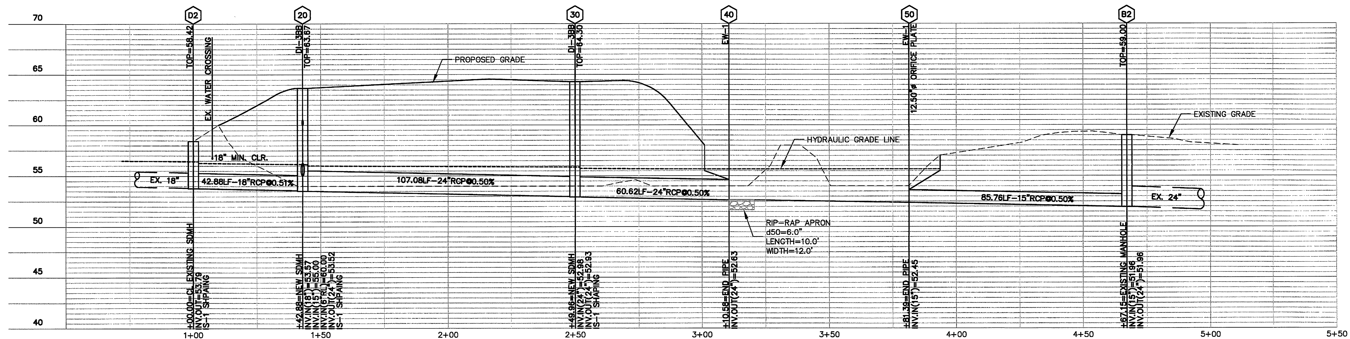
STORM SEWER PROFILES
