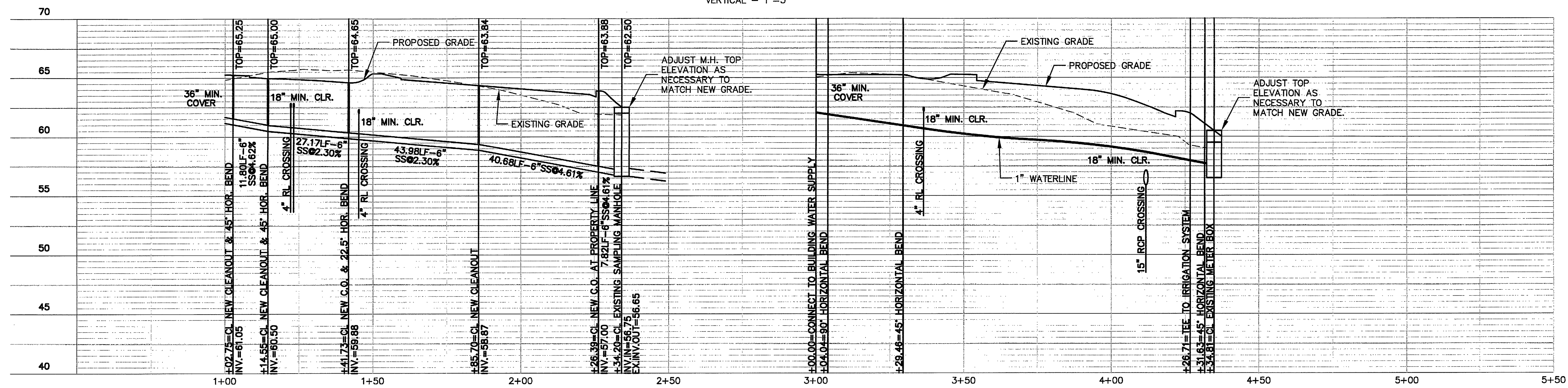
SANITARY SEWER PROFILE
