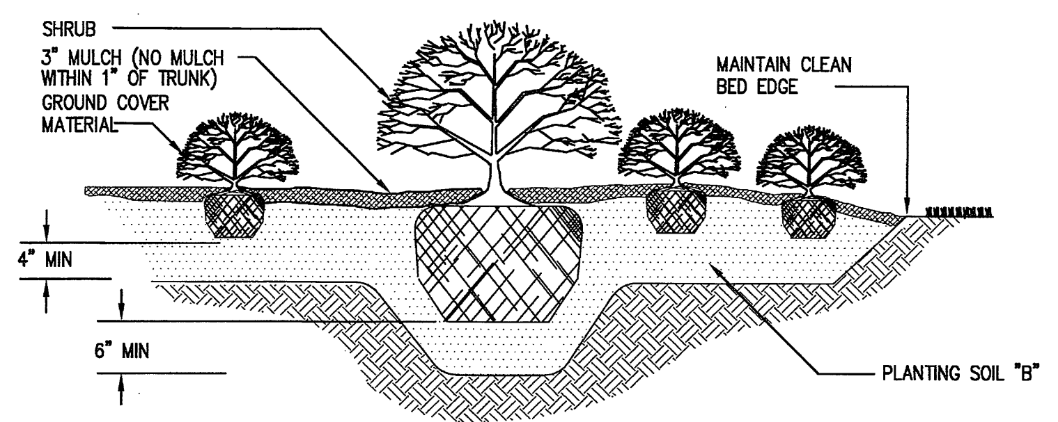
TYPICAL GROUND COVER & SHRUB BED DETAIL N.T.S.
