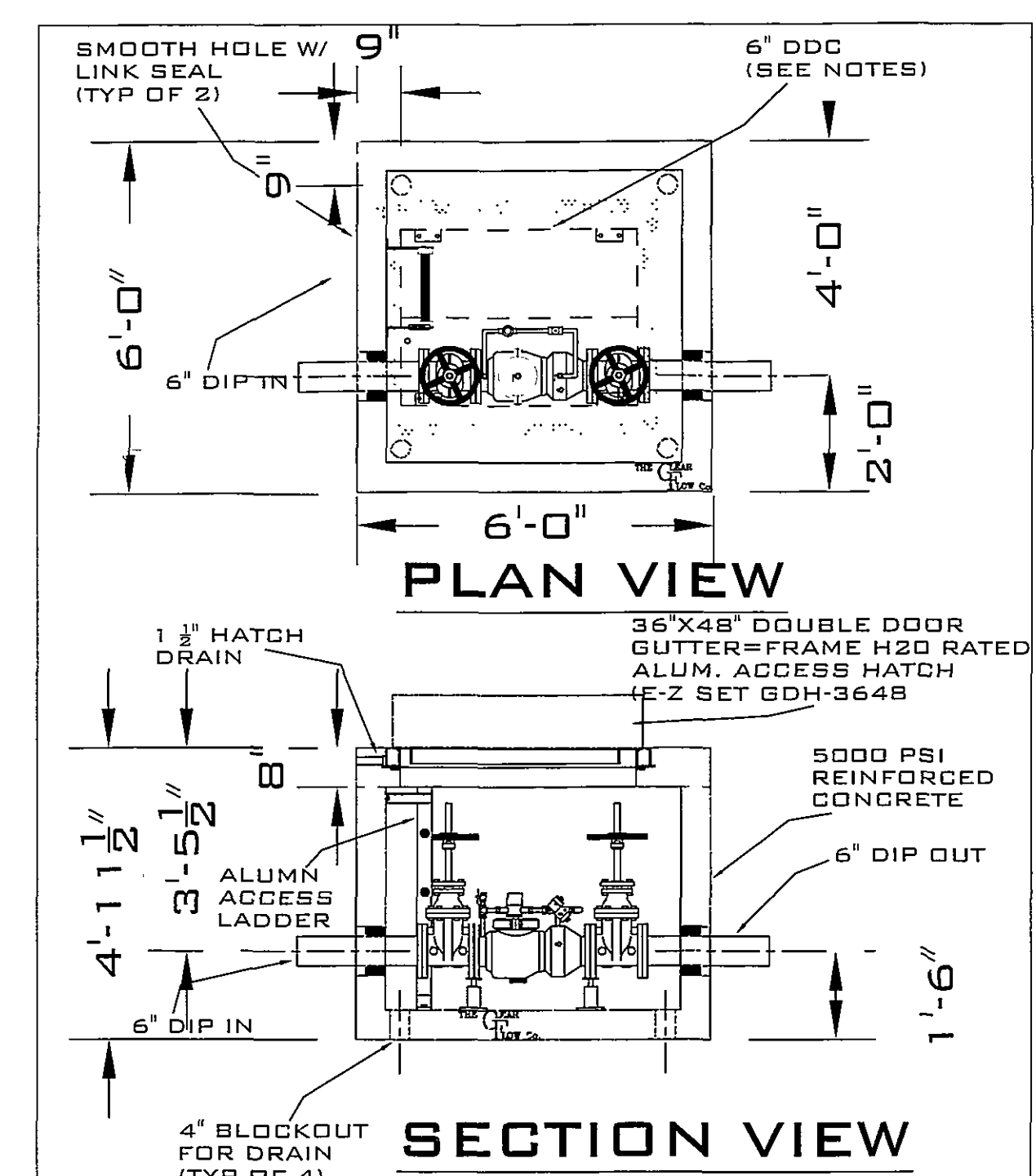
FREE STANDING F.D.C. DETAIL 1/2" = 1'-0"
