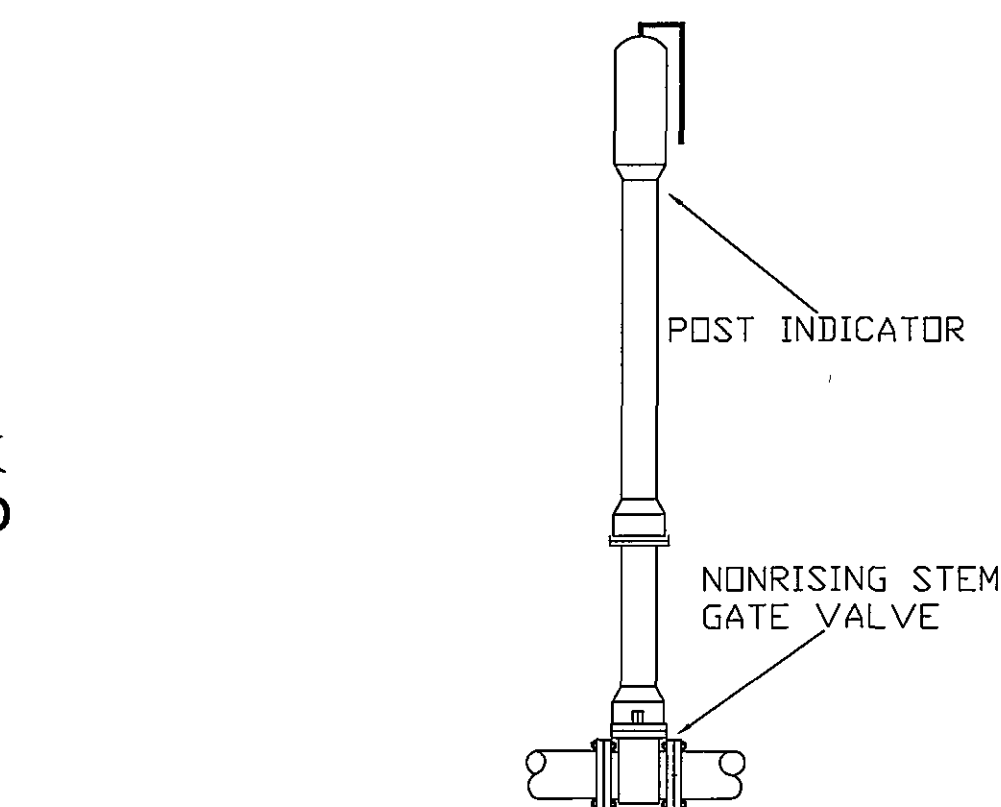
POST INDICATOR VALVE DETAIL 1/2" = 1'-0"
