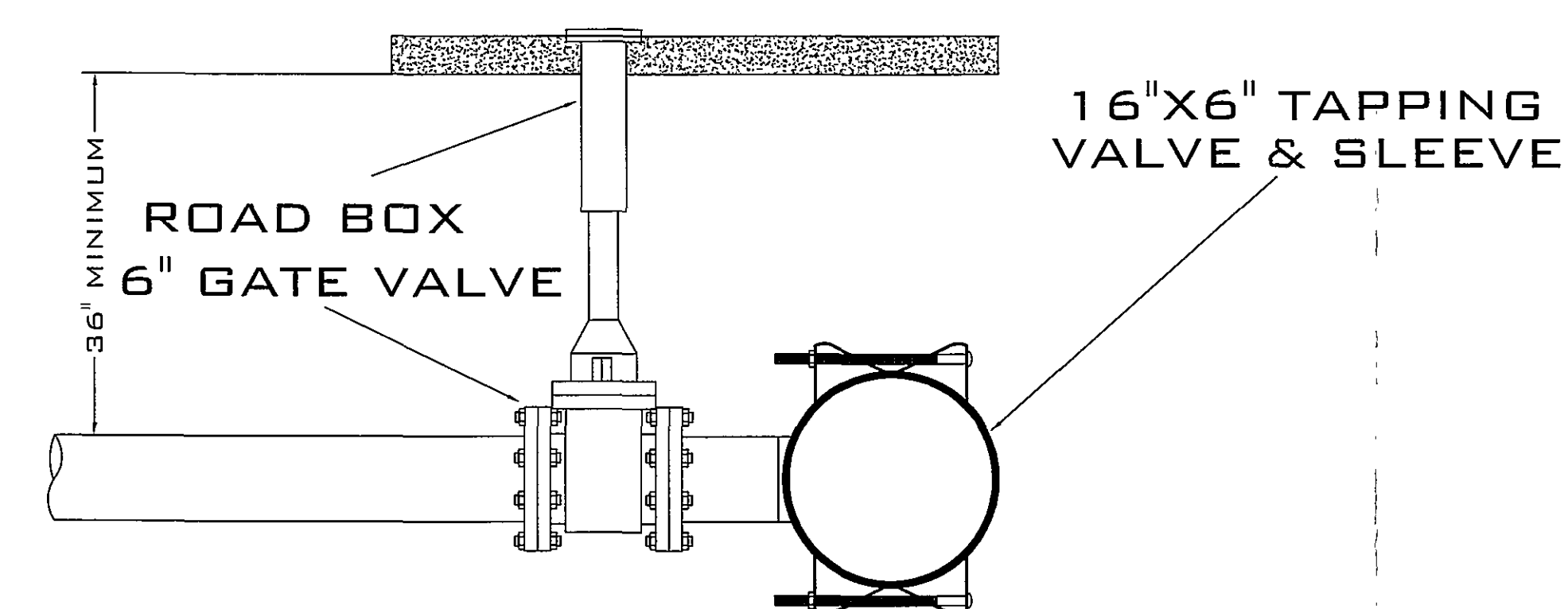
TAPPING VALVE & SLEEVE \frac{1}{2}'' = 1'-0''
