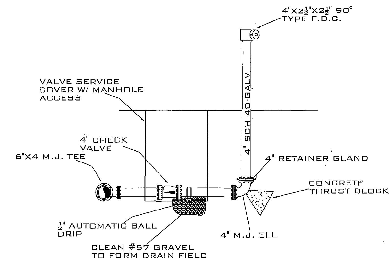
FREE STANDING F.D.C. DETAIL 1/2" = 1'-0"
