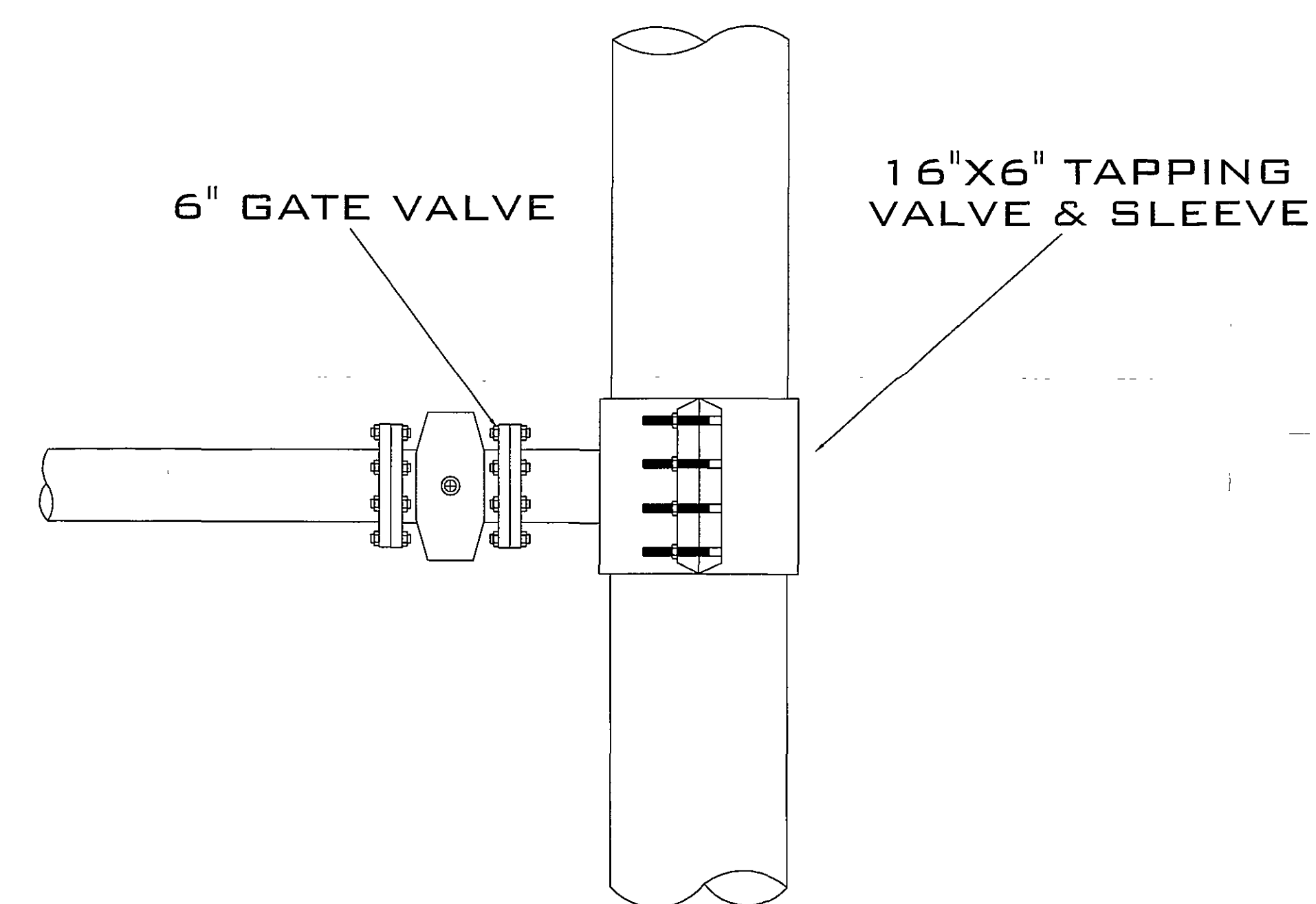
TAPPING VALVE & SLEEVE 1/2" = 1'-0"
