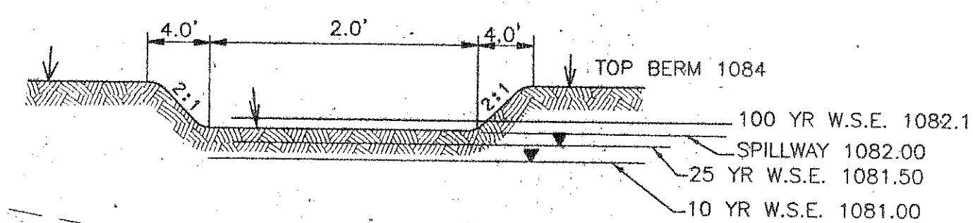
EMERGENCY SPILLWAY DETAIL NO SCALE
