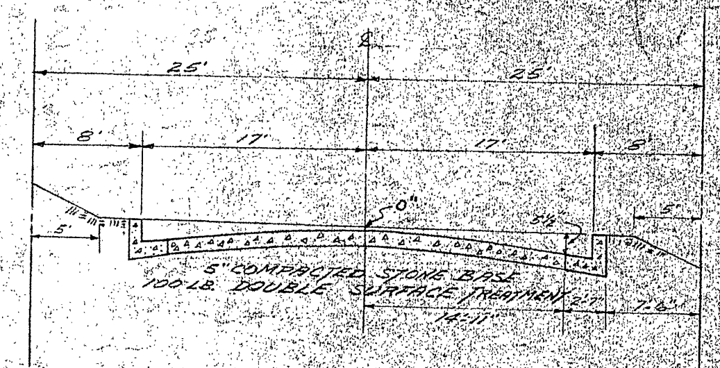
TYP. CROSS SECTION OF 50 FOOT STREET WITH CURB 1/8" SCALE
