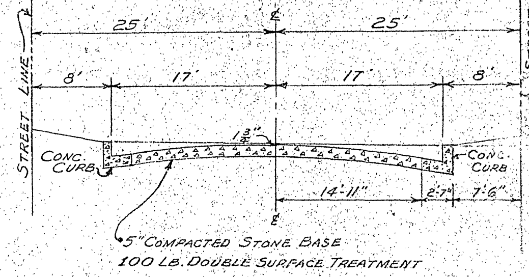
TYPICAL CROSS SECTION - 50' STREET NO SCALE
