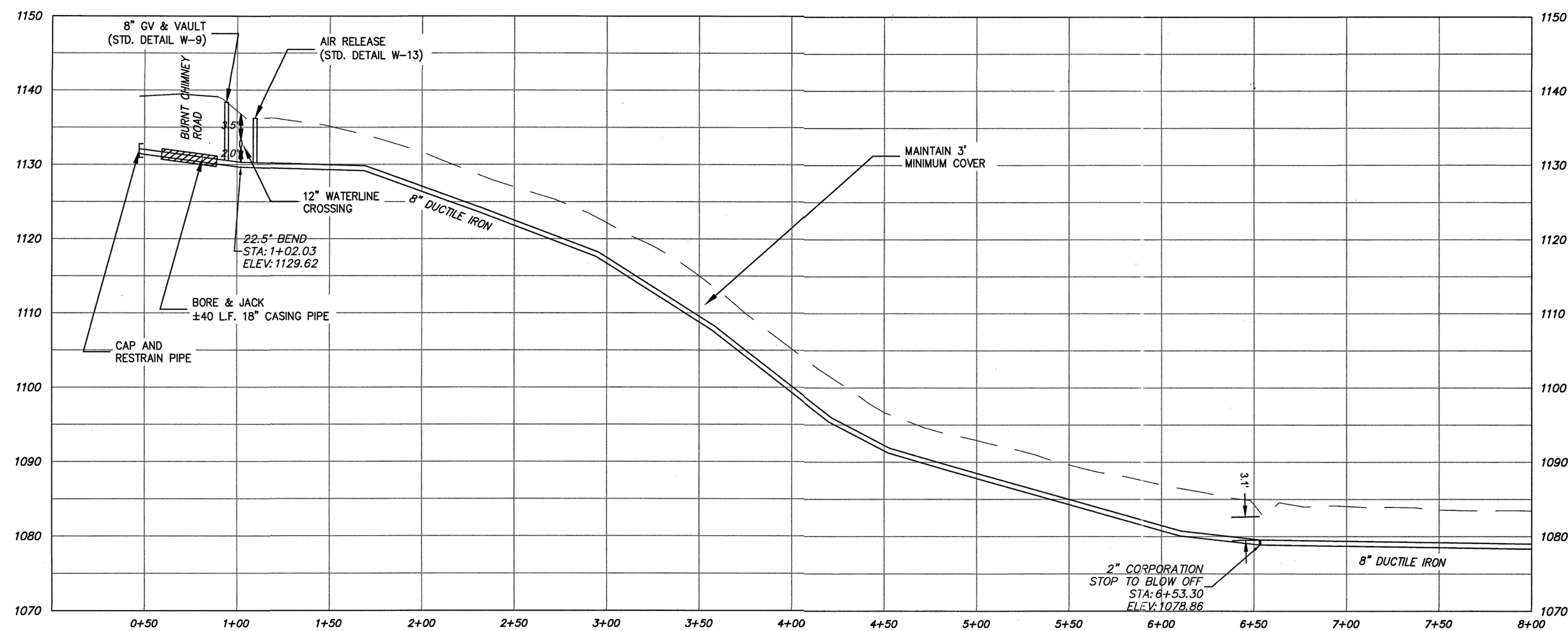
WATERLINE PROFILE 1" = 40' Horizontal 1" = 10' Vertical
