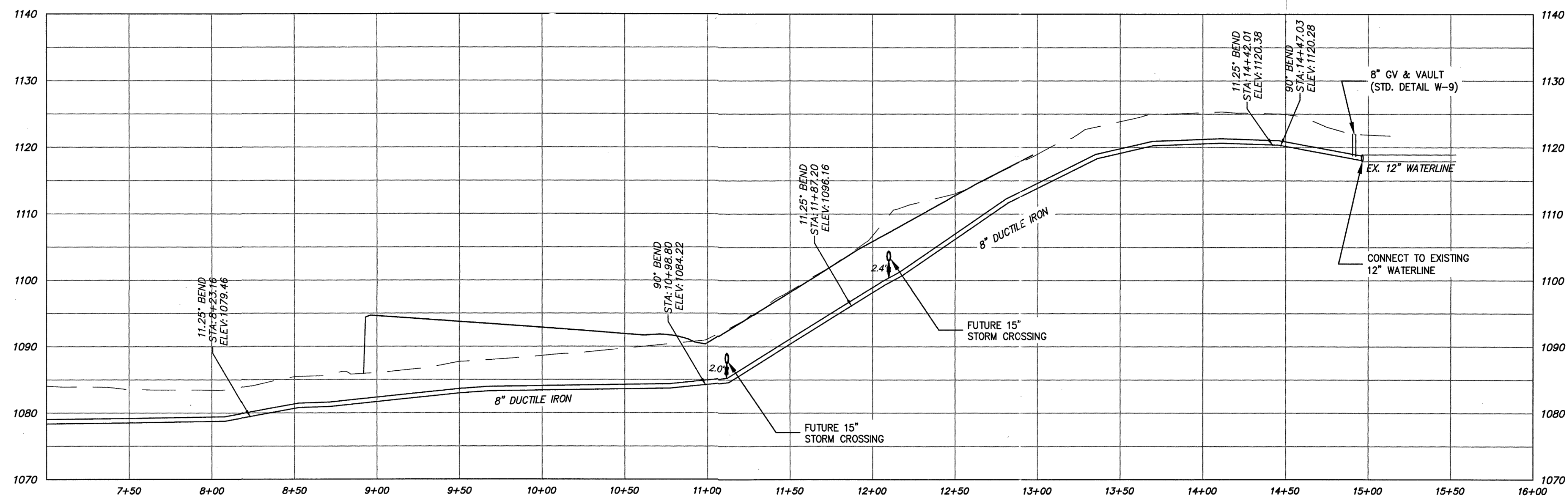
WATERLINE PROFILE 1" = 40' Horizontal 1" = 10' Vertical
