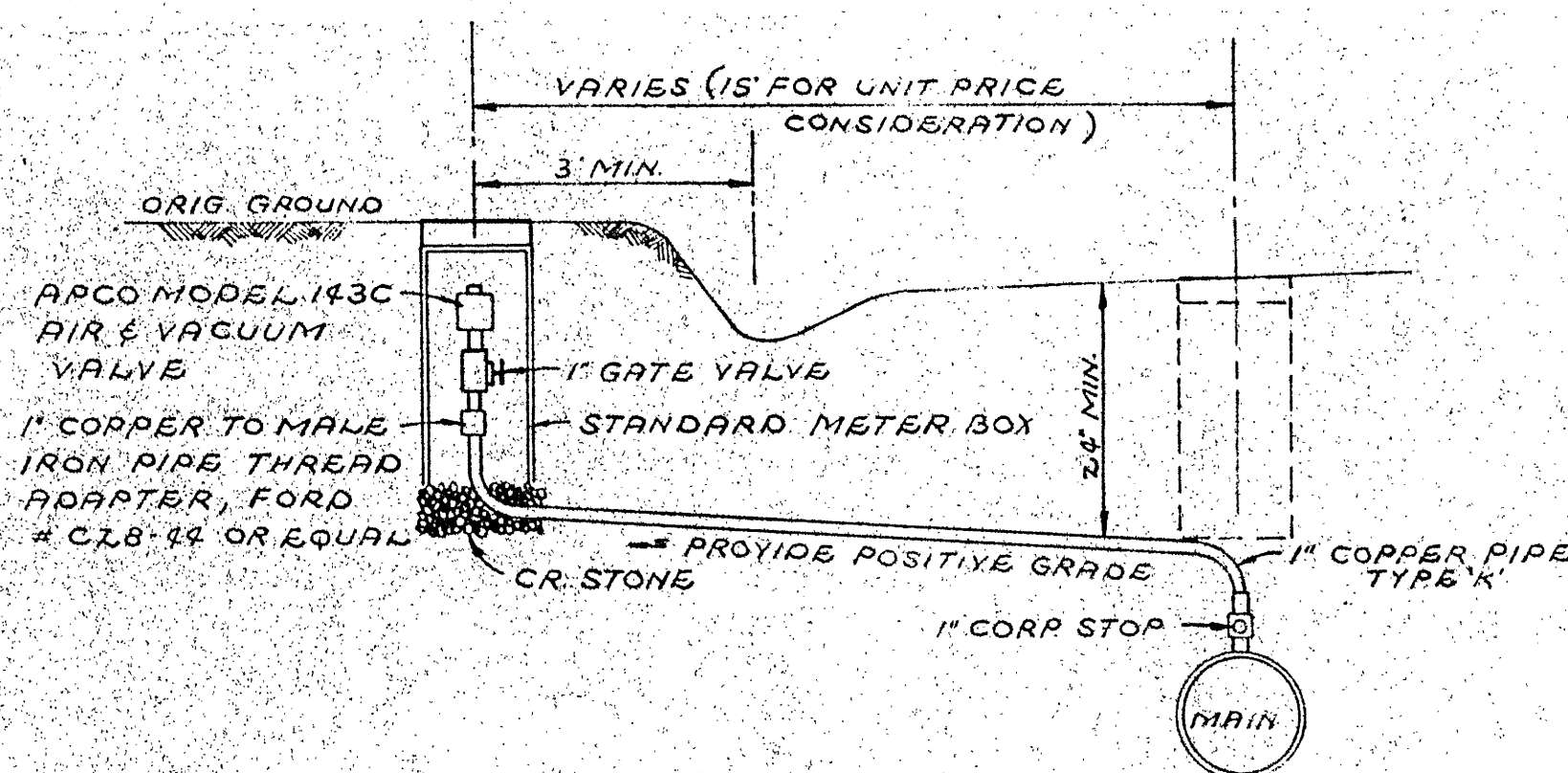
AIR RELEASE VALVE DETAIL
