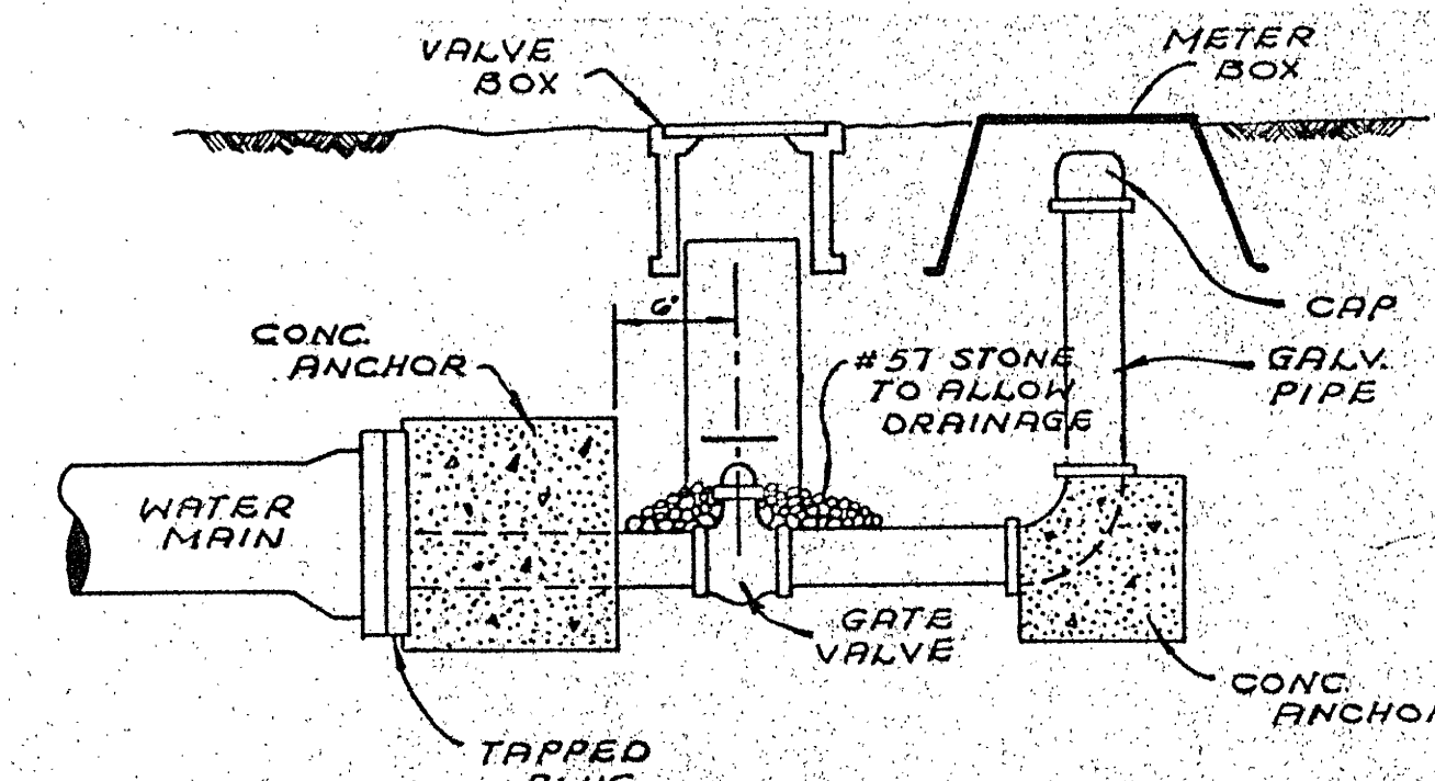
BLOW-OFF VALVE ASSEMBLY
