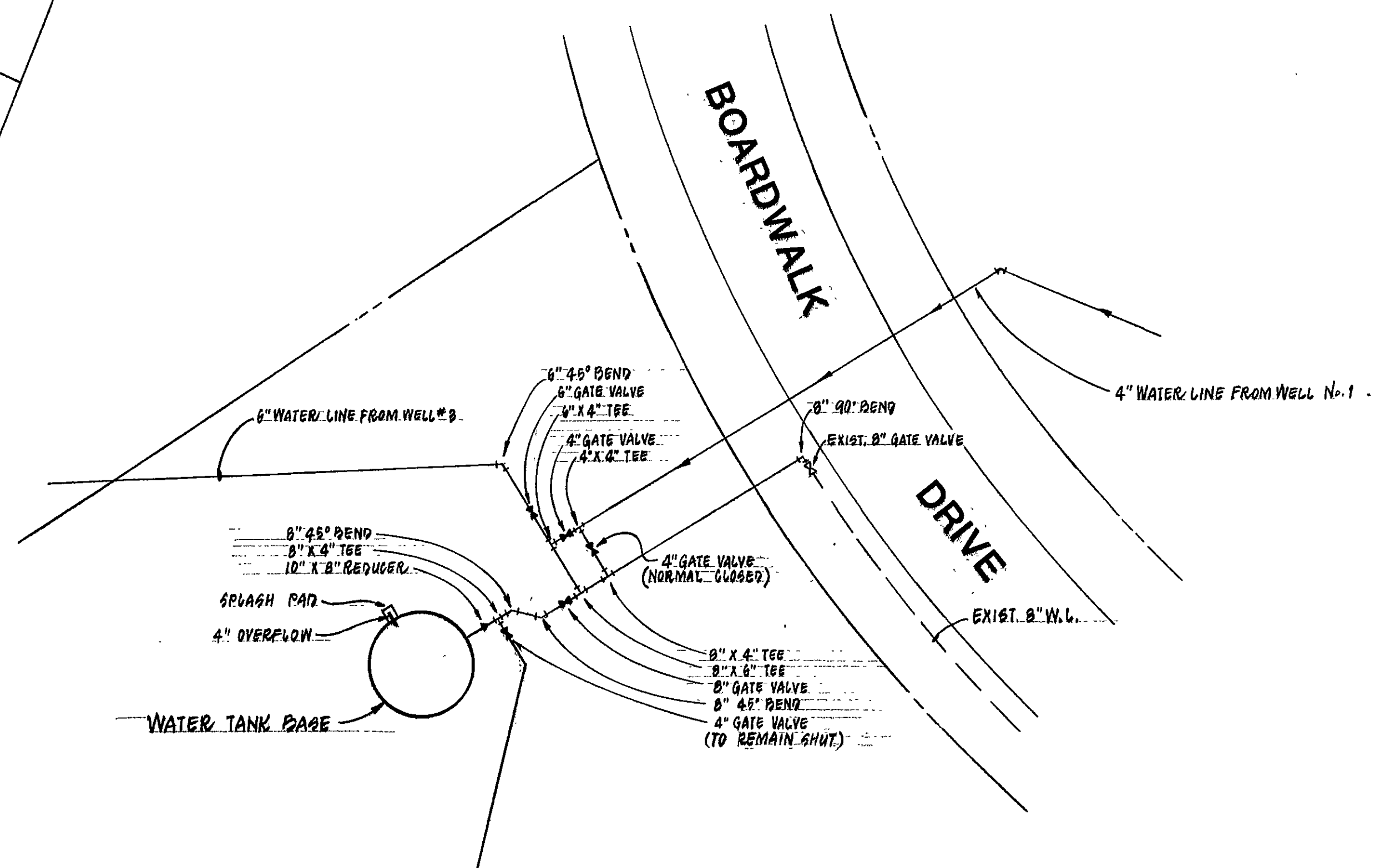
TANK PIPING DETAIL Scale: 1" = 20'
