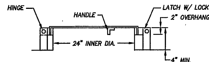
ROOF MANHOLE NO SCALE
