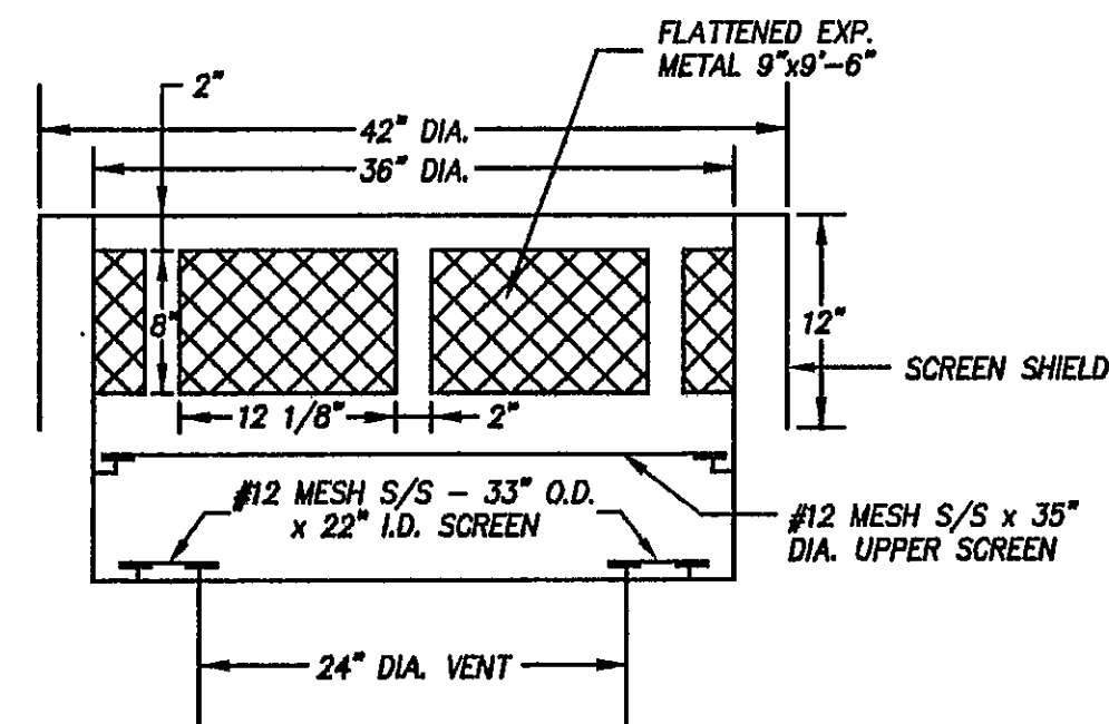
SCREENED VENT DETAIL NO SCALE
