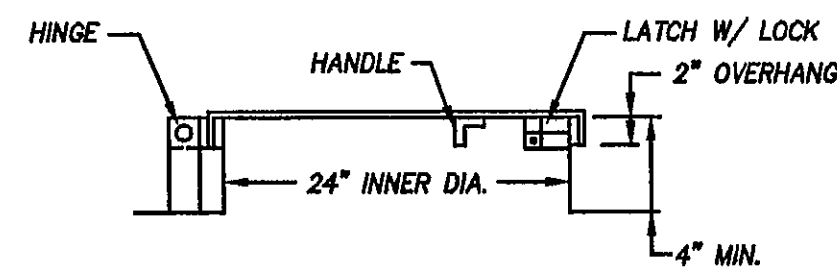
ACCESS TUBE ROOF MANHOLE NO SCALE
