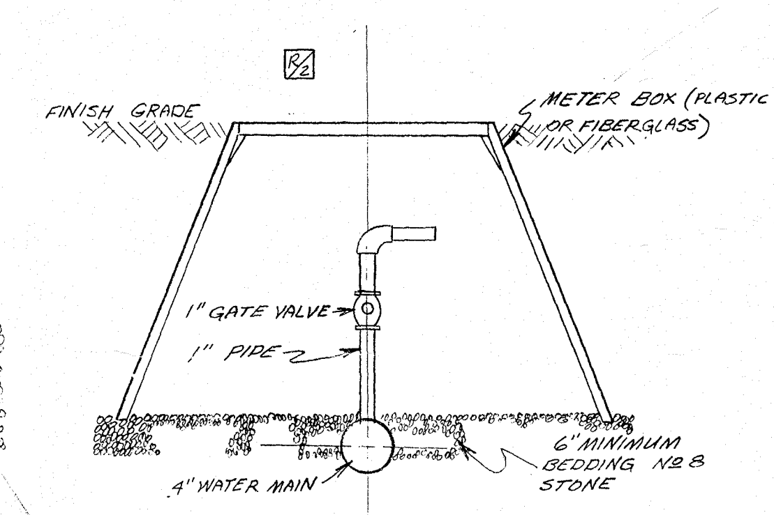
MANUAL AIR RELEASE ASSEMBLY NO SCALE
