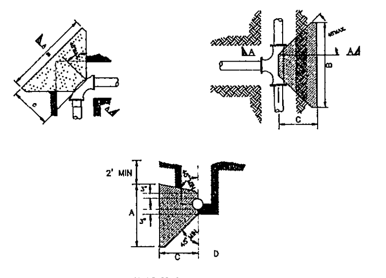
THRUST BLOCK FOR HORIZONTAL & LOWER VERTICAL BENDS
