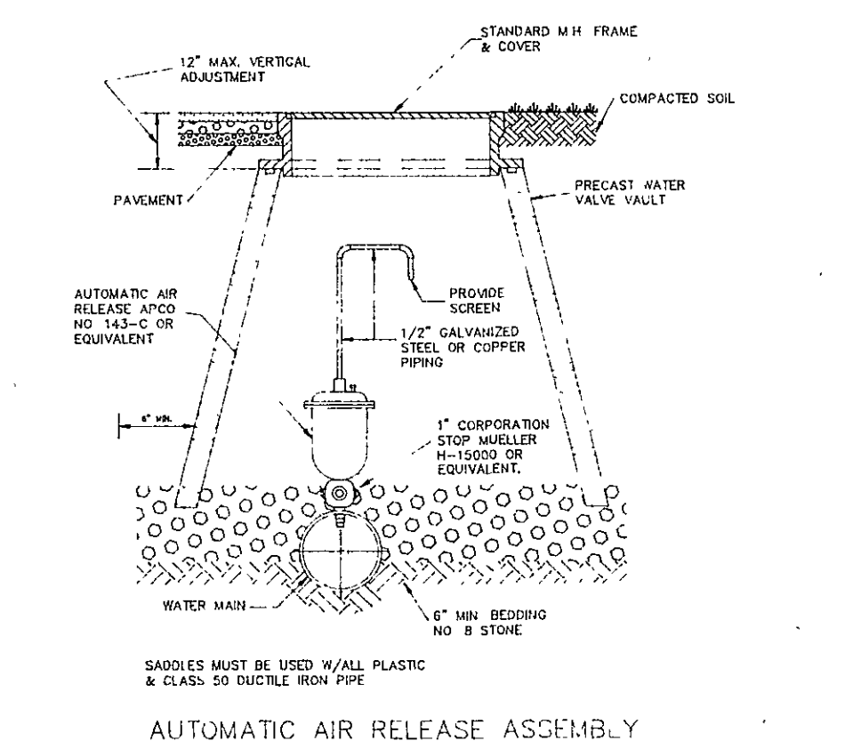
AUTOMATIC AIR RELEASE ASSEMBLY
