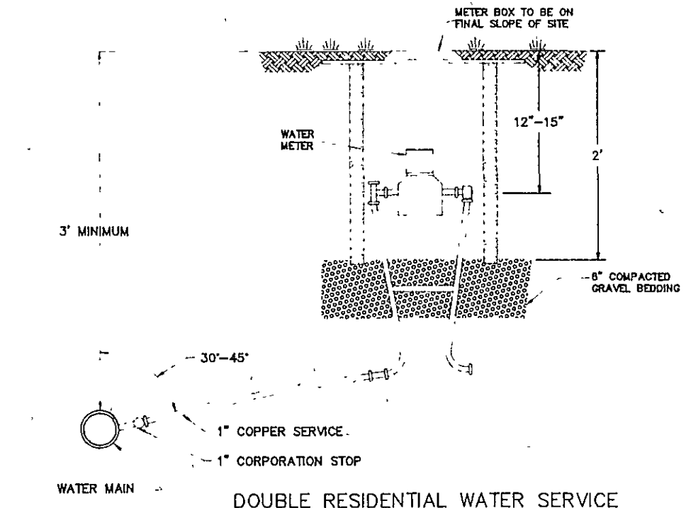
DOUBLE RESIDENTIAL WATER SERVICE
