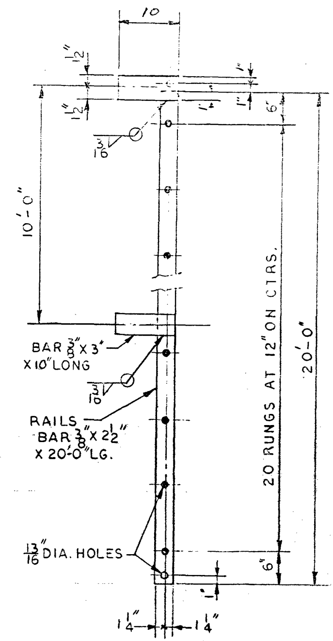
DETAIL - STANDARD 20'-0" LADDER SECTION (39'-0") REQ'D. FOR INTERIOR LADDER
