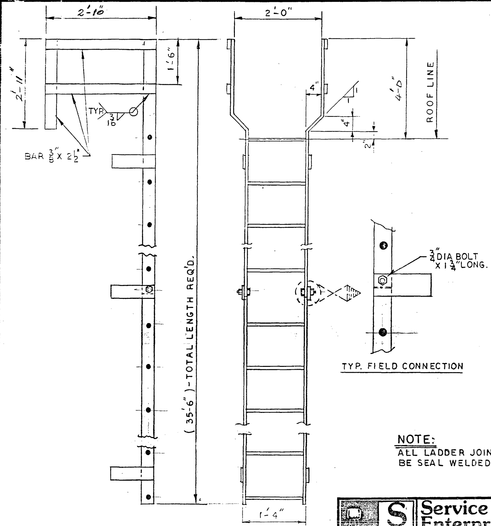
DETAIL - EXTERIOR SHELL LADDER
