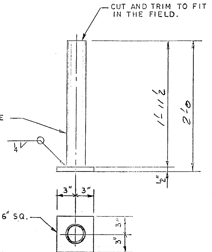
DETAIL - PIPE SUPPORT
