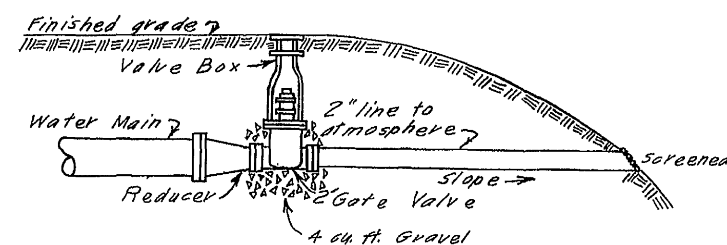
BLOWOFF Not to Scale
