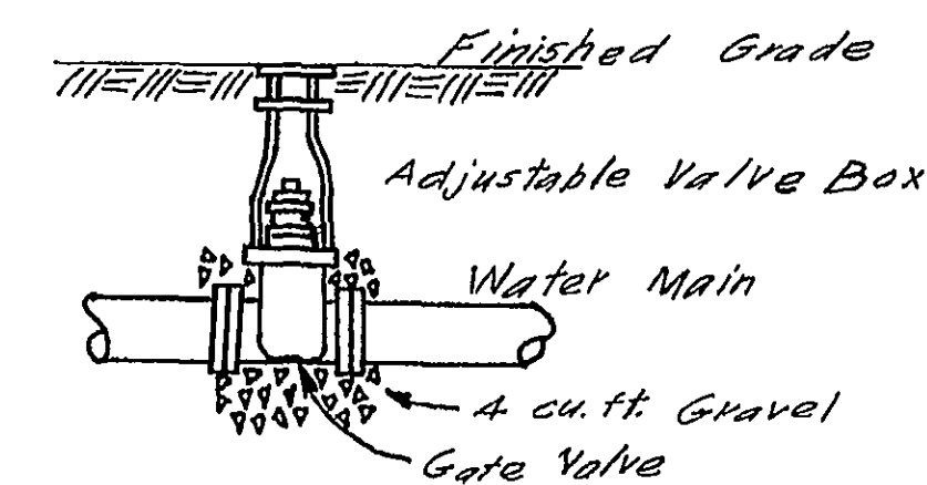
VALVE INSTALLATION
