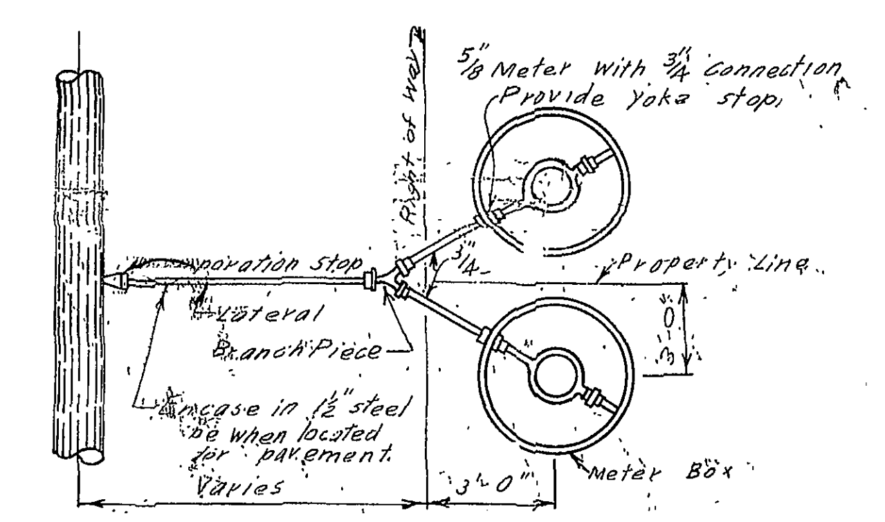
WATER SERVICE CONNECTIONS Not to Scale
