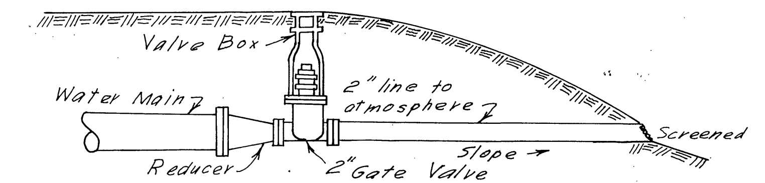
BLOWOFF Not to Scale
