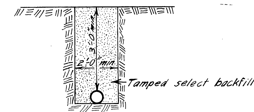
PIPE BEDDING DETAIL Not to Scale
