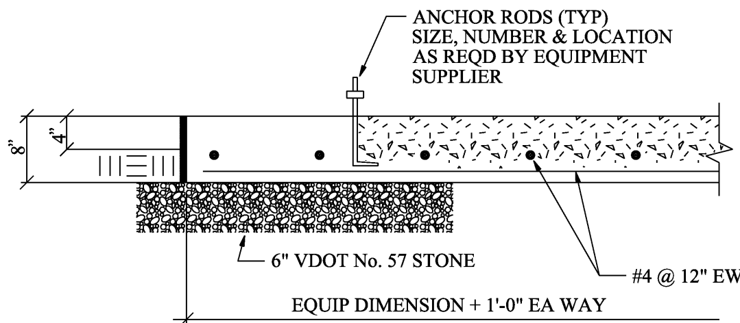
GENERATOR BASE DETAIL
