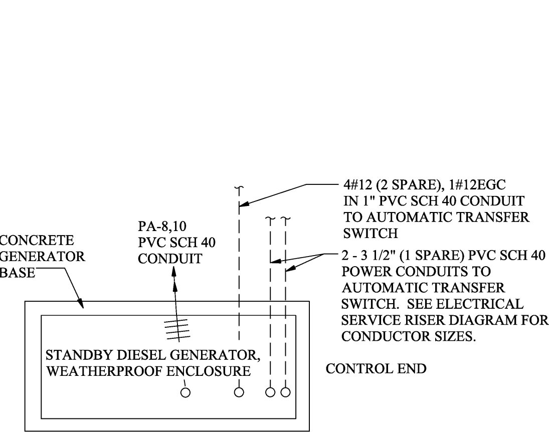
GENERATOR PLAN
