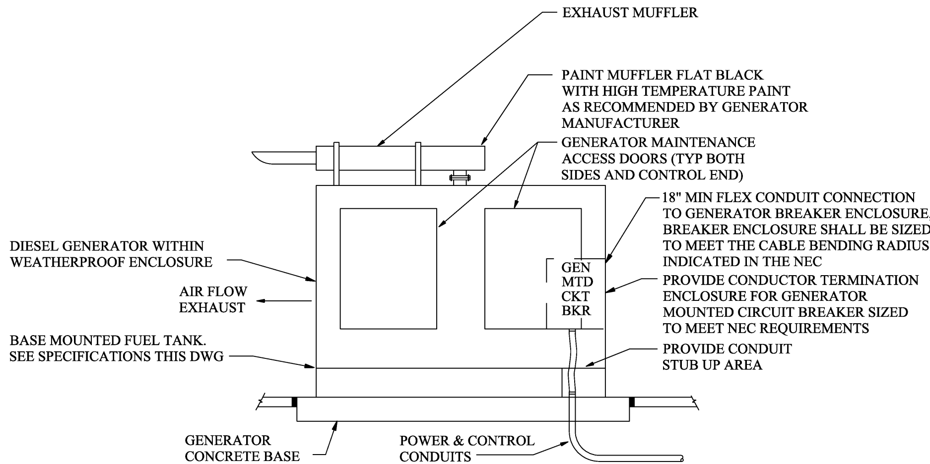
GENERATOR ELEVATION
