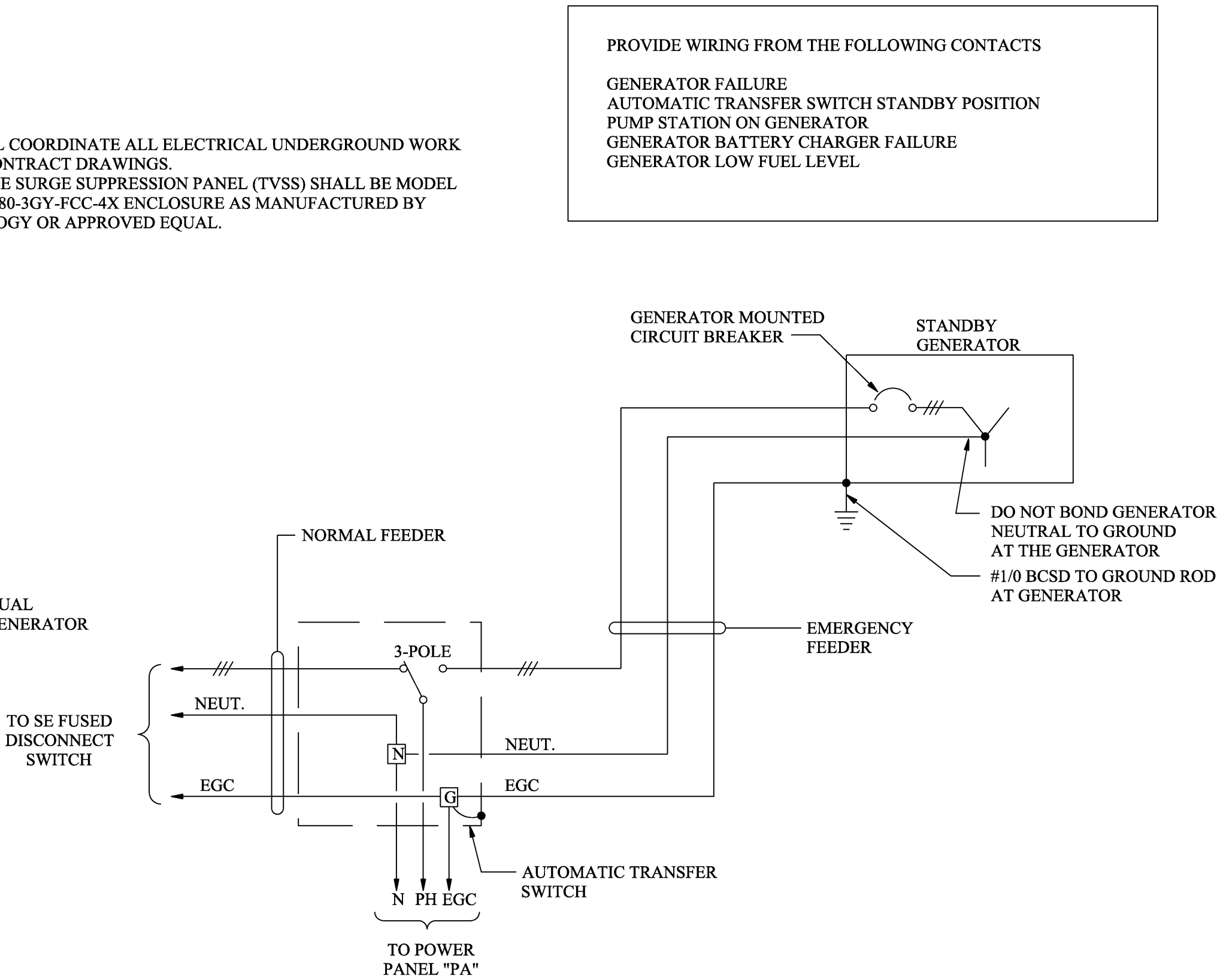
CONNECTION DIAGRAM - NEUTRAL & GROUND CONDUCTORS
