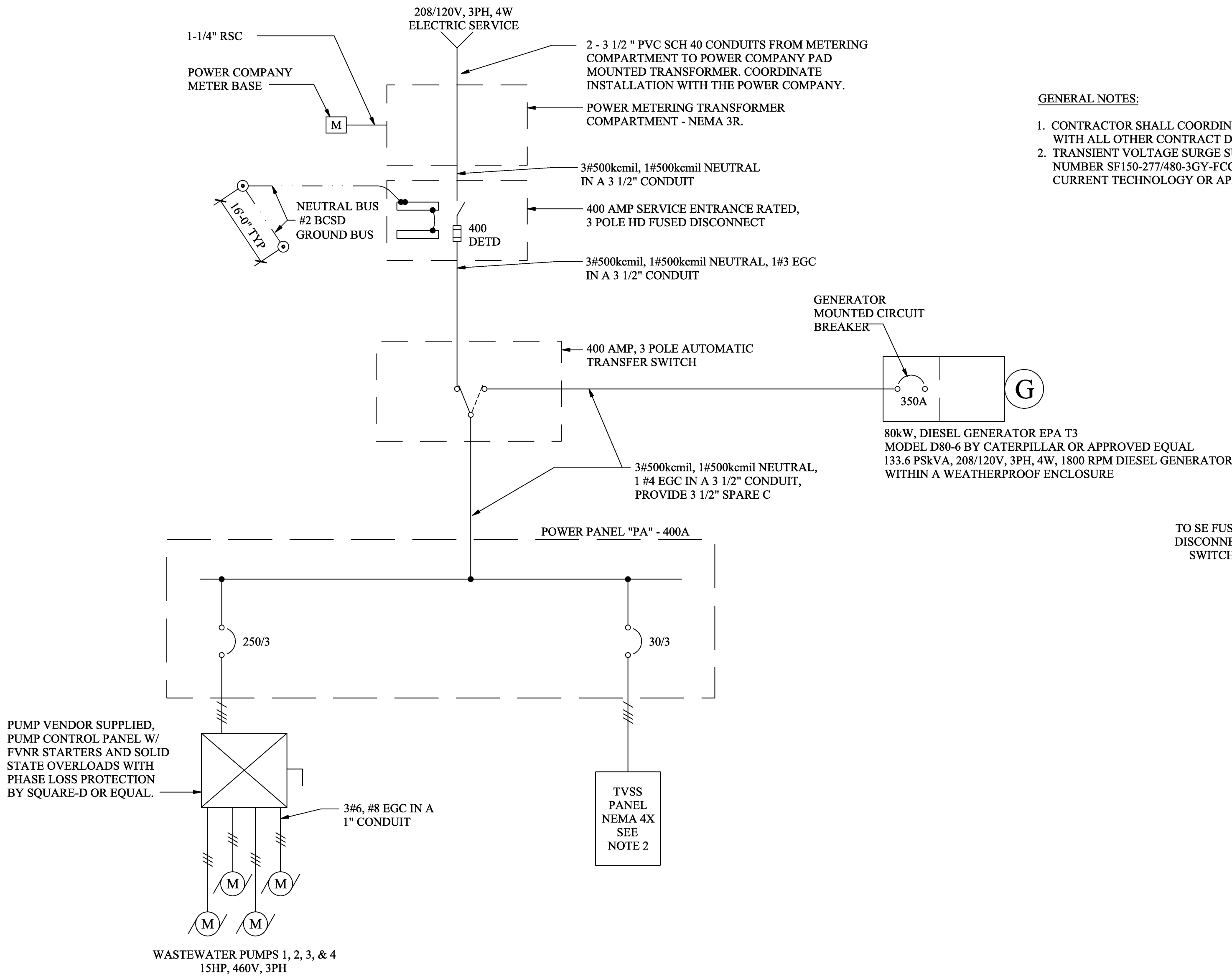
PUMP STATION ELECTRICAL SERVICE - RISER DIAGRAM
