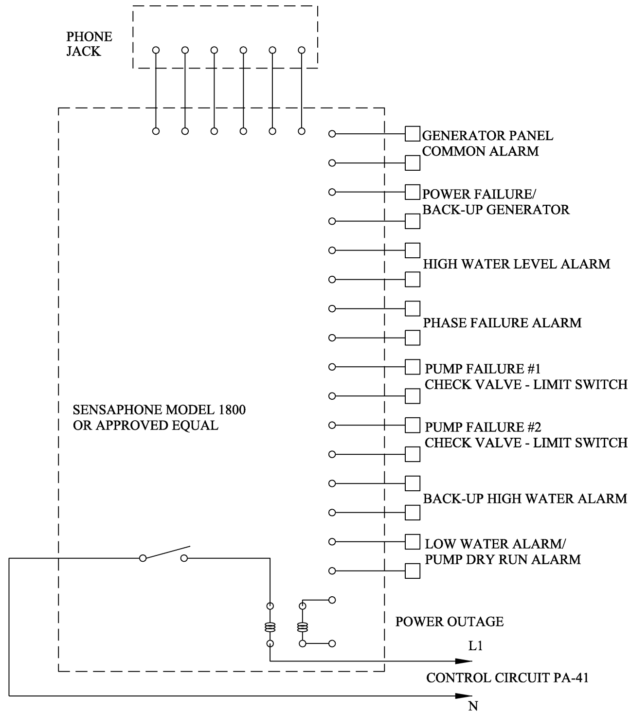
PUMP STATION SCHEMATIC AUTO DIALER
