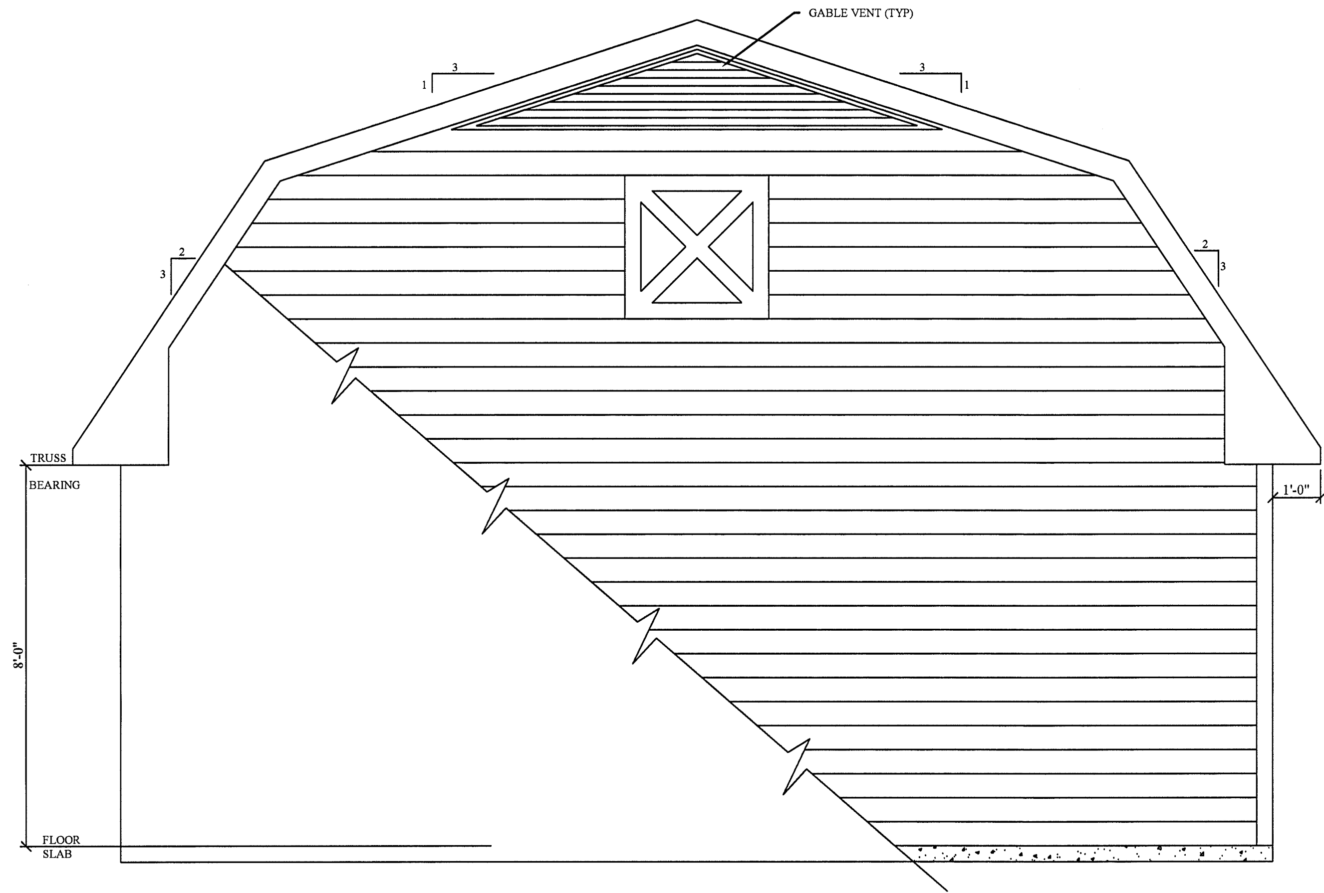
SOUTH ELEVATION SCALE: 1/2" = 1'-0"
