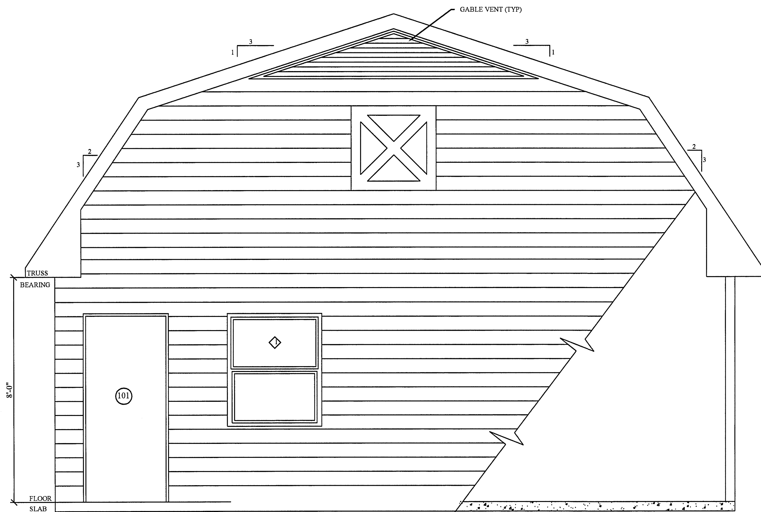
NORTH ELEVATION SCALE: 1/2" = 1'-0"
