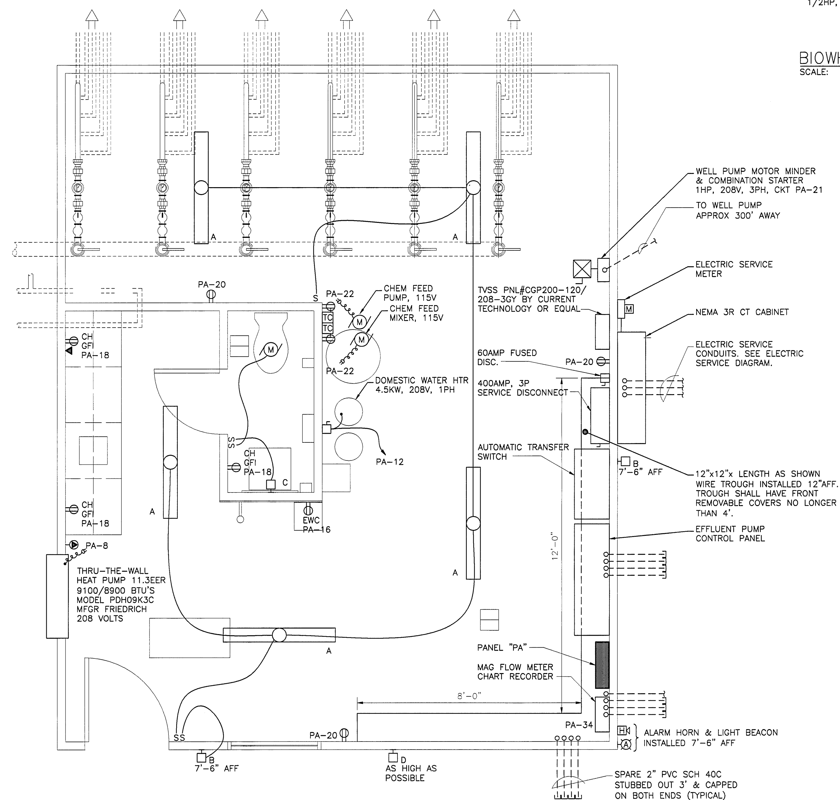
LAB BLDG POWER & LIGHTING FLOOR PLAN SCALE: 1/2" = 1'-0"
