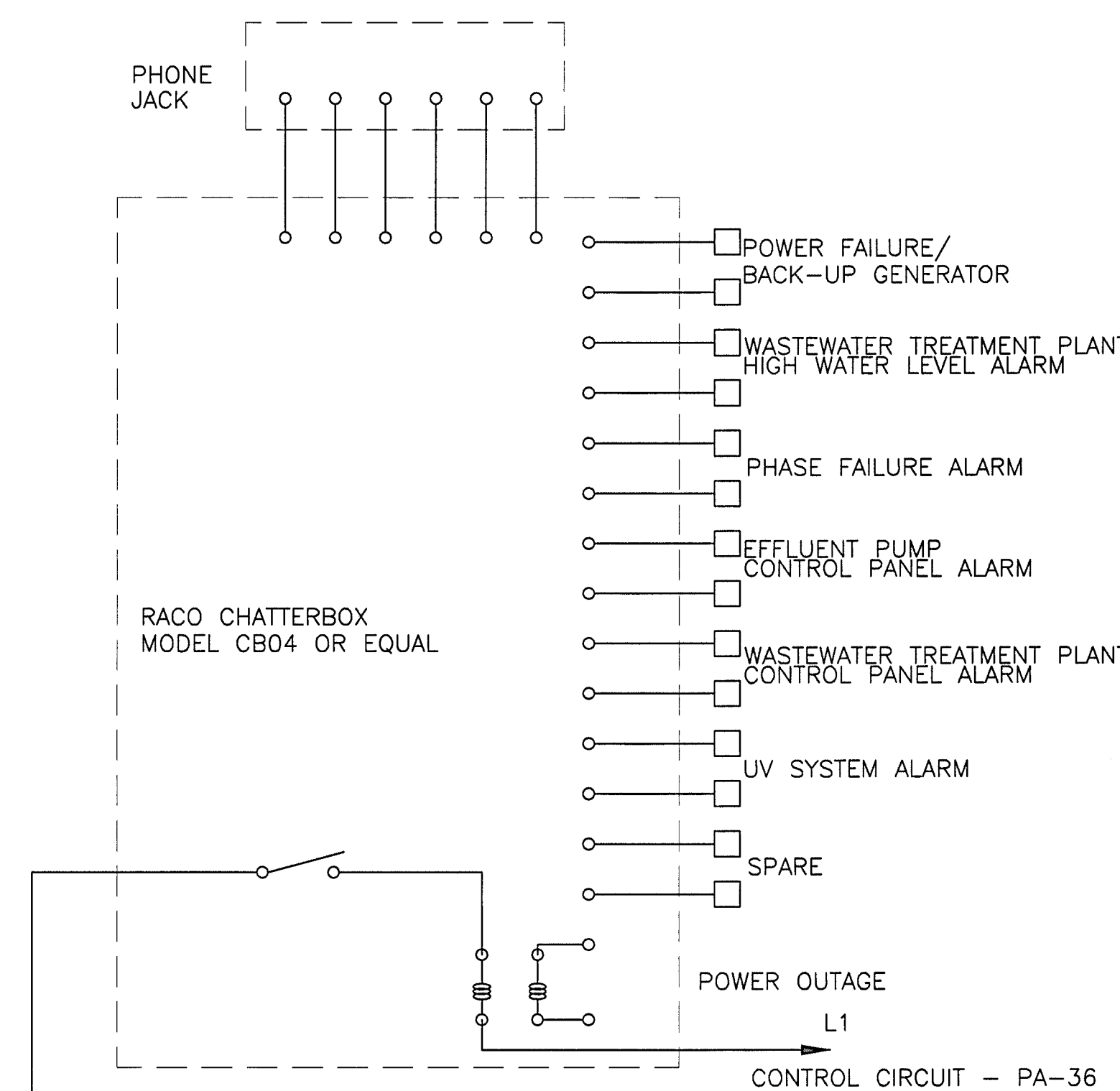
WASTEWATER TREATMENT PLANT SCHEMATIC AUTO DIALER
