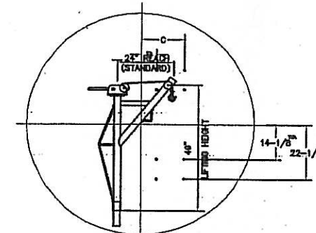
PORTABLE HOIST
