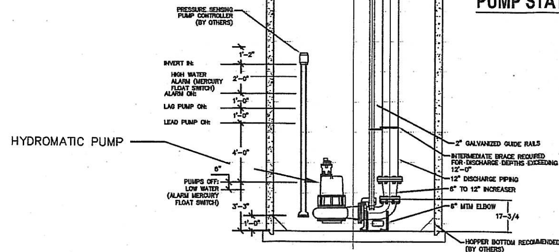
PUMP STATION SECTION
