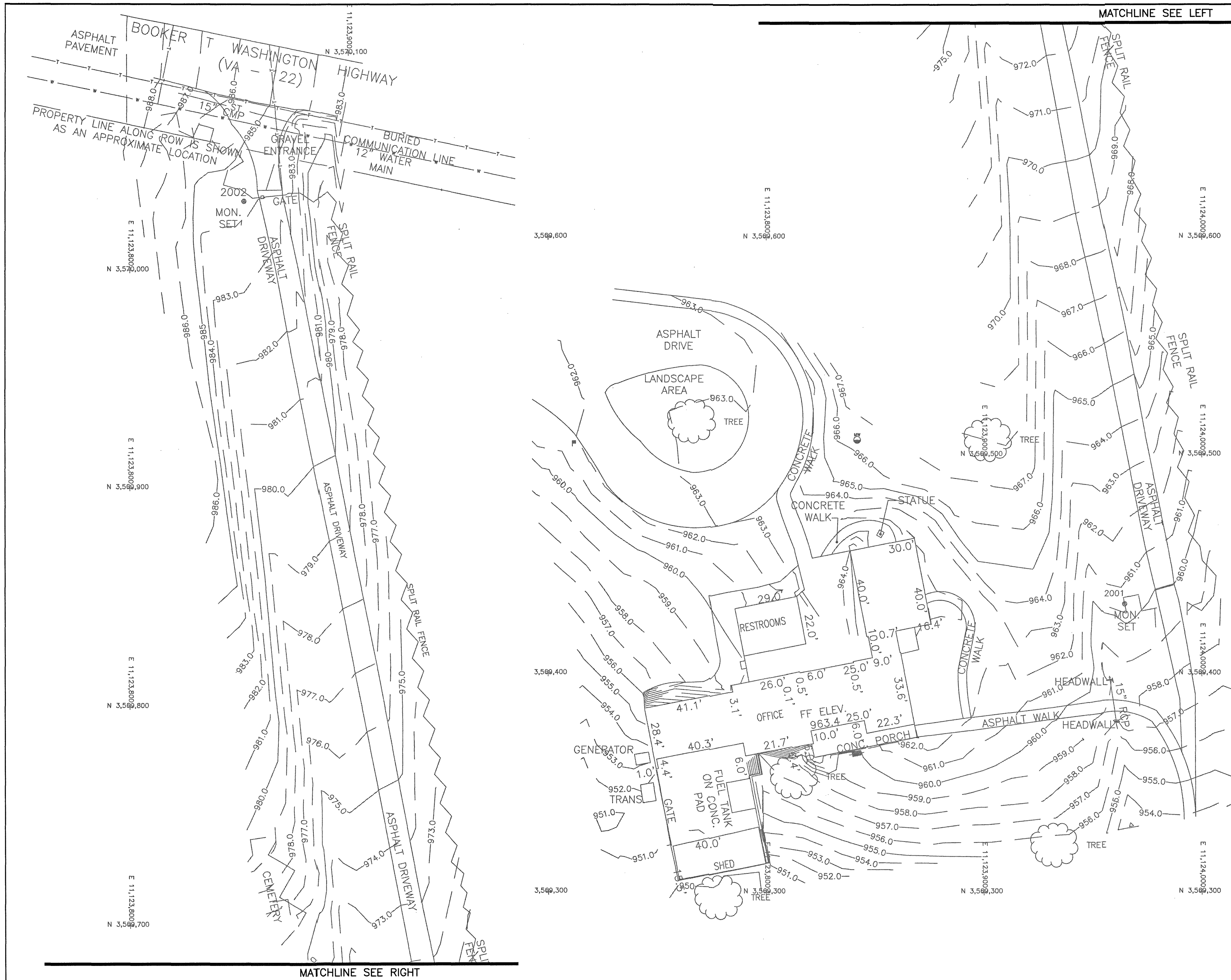
1 EXISTING CONDITIONS PLAN C1 SCALE: 1"=25'
