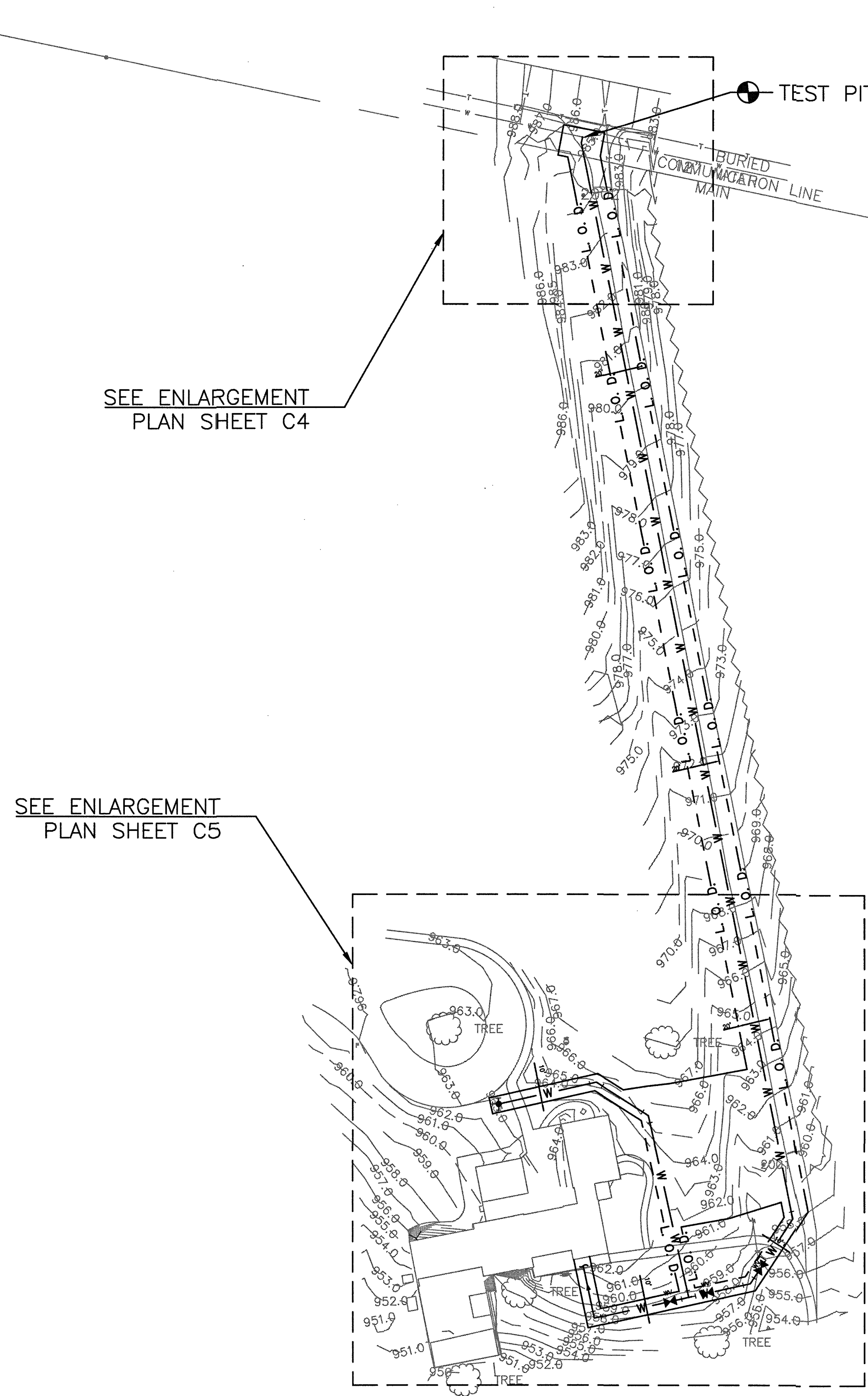
1 OVERALL SITE PLAN C3 SCALE: 1"=50'
