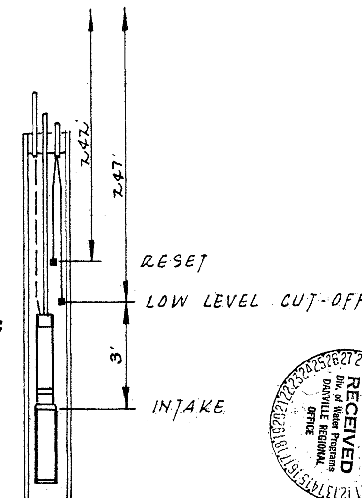
PUMP CONTROLS SCHEMATIC
