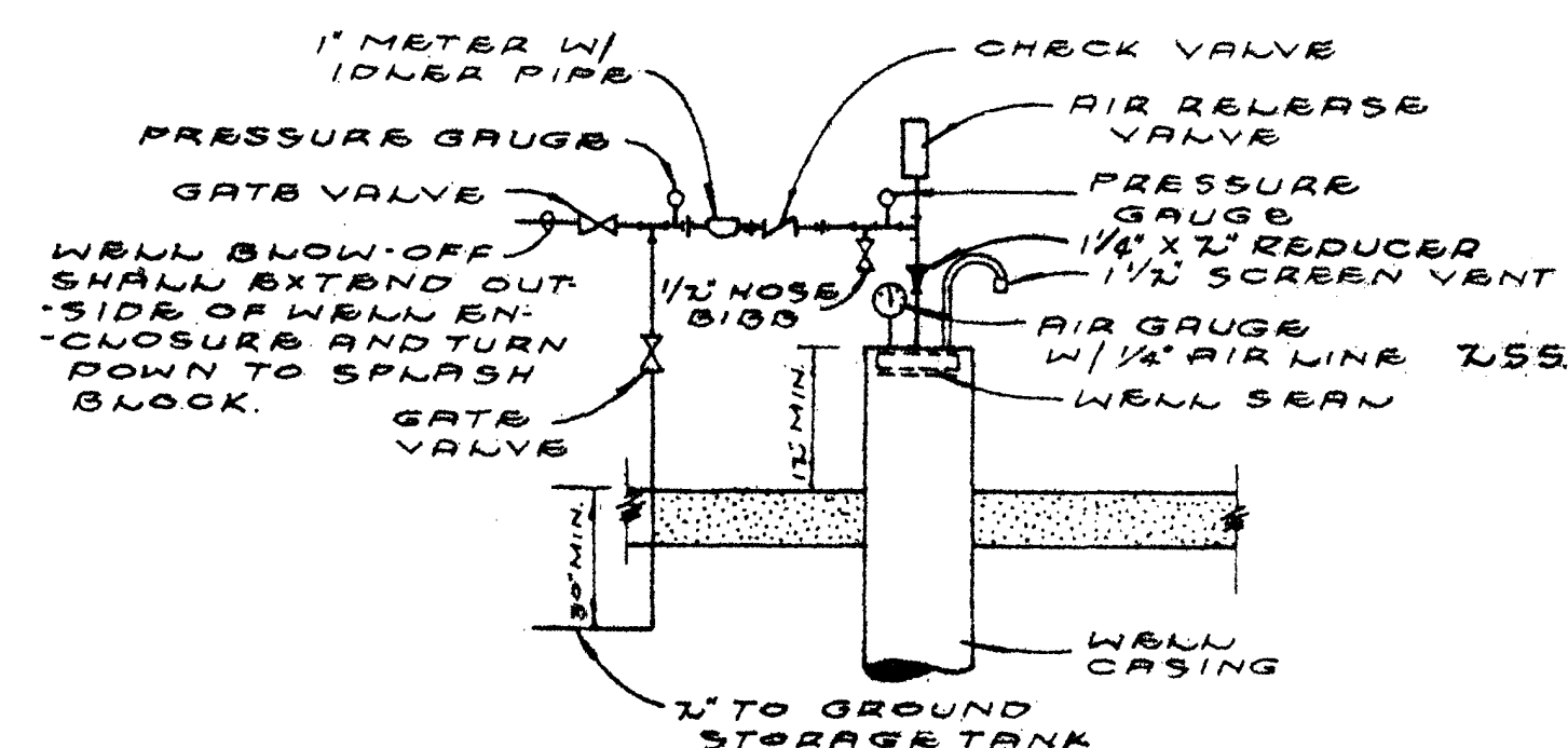
WELL DETAIL
