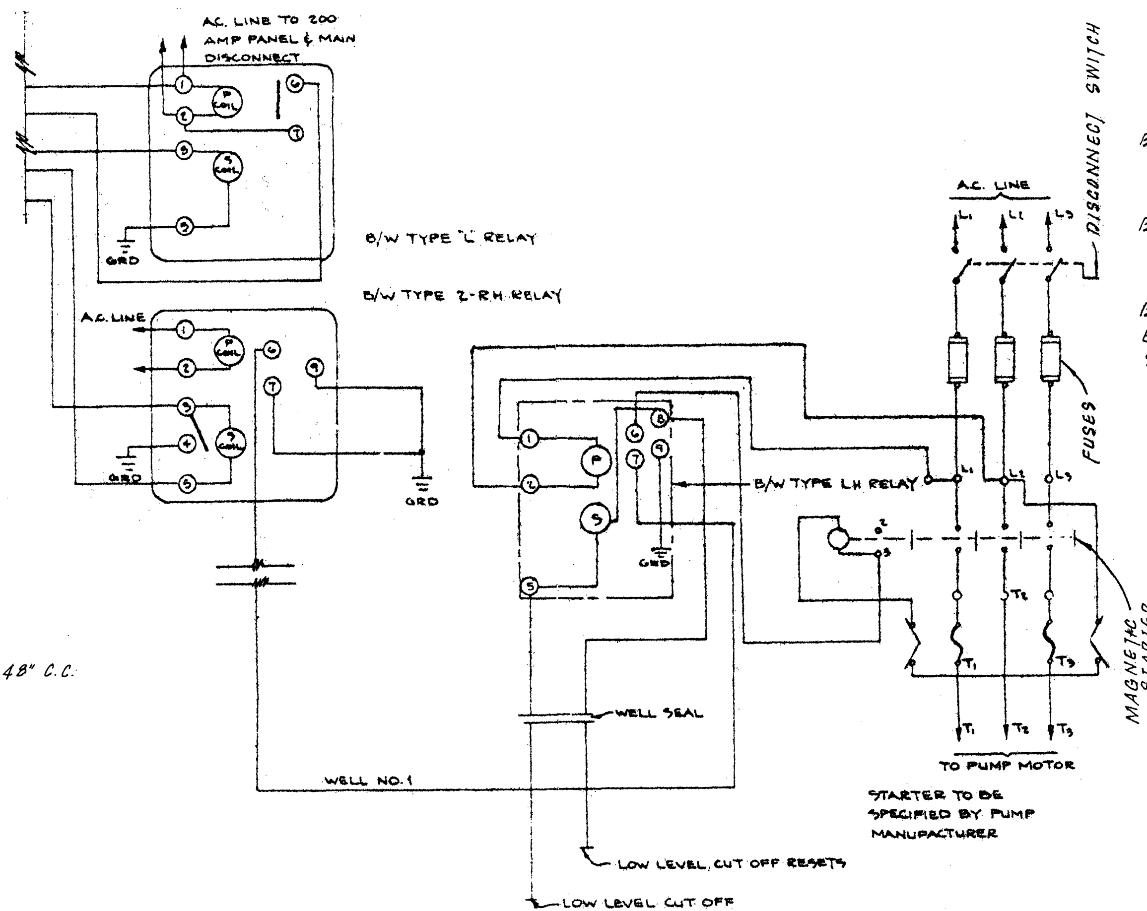
TYPICAL CONTROLS AT WELL
