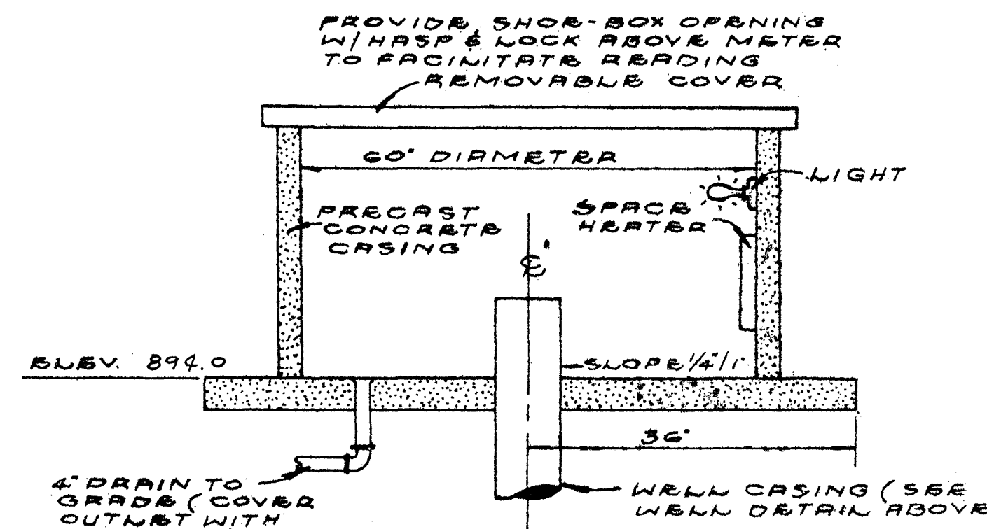
WELL HOUSING DETAIL
