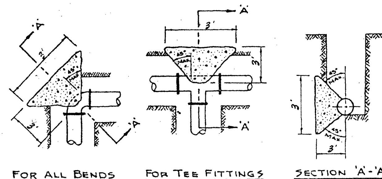
TYPE 'F' ANCHOR
