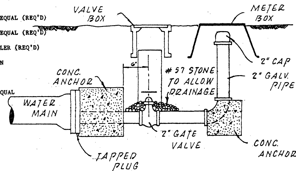
2" BLOW-OFF ASSEMBLY
