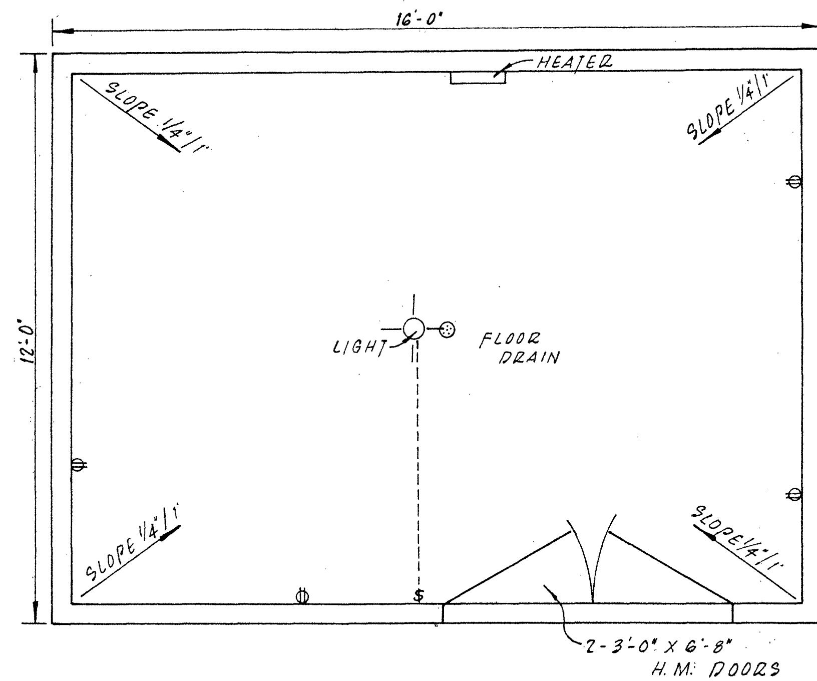
PUMP HOUSE PLAN
