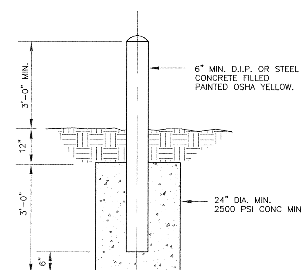
BOLLARD DETAIL
