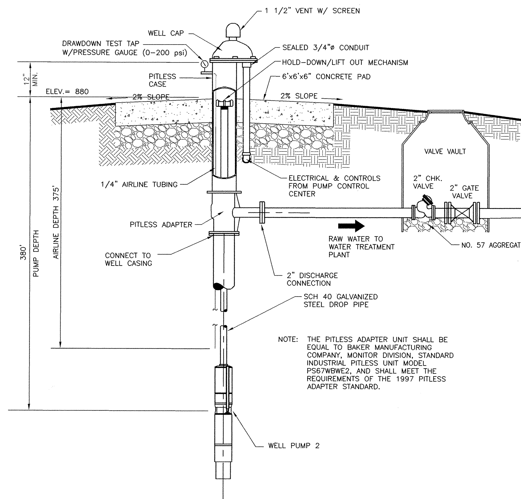
SECTION - WELL 2 NOT TO SCALE
