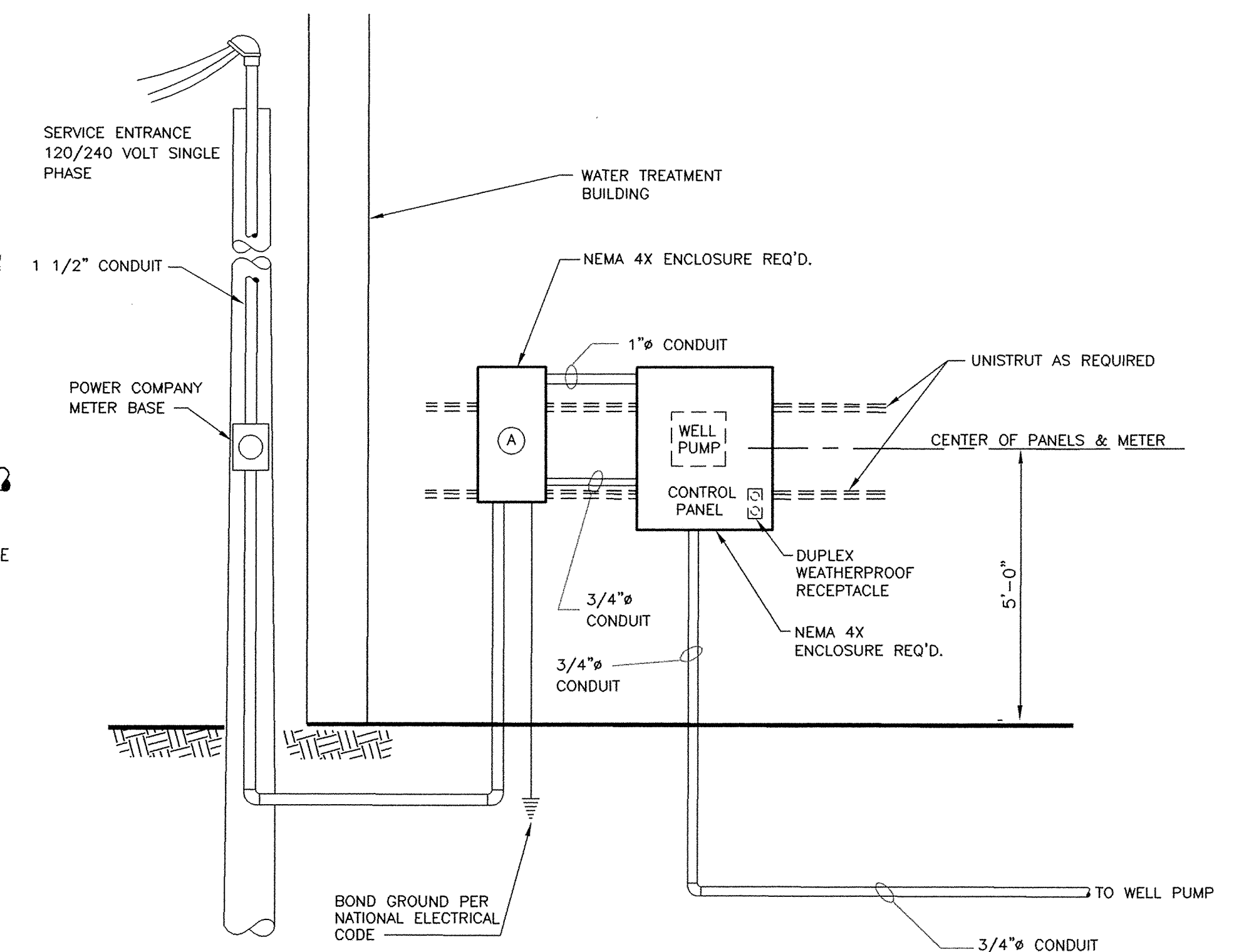
④ ELECTRICAL/STRUCTURAL PUMP CONTROL CENTER NOT TO SCALE
