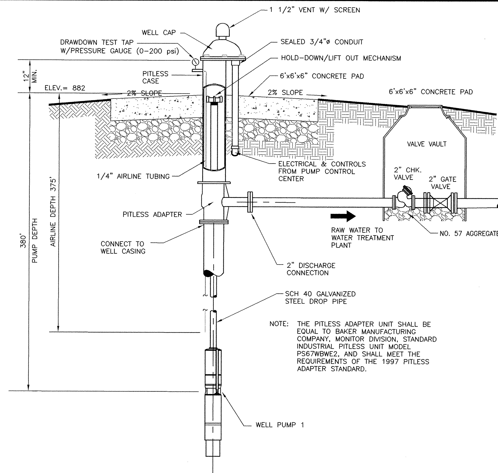
SECTION - WELL 1 NOT TO SCALE
