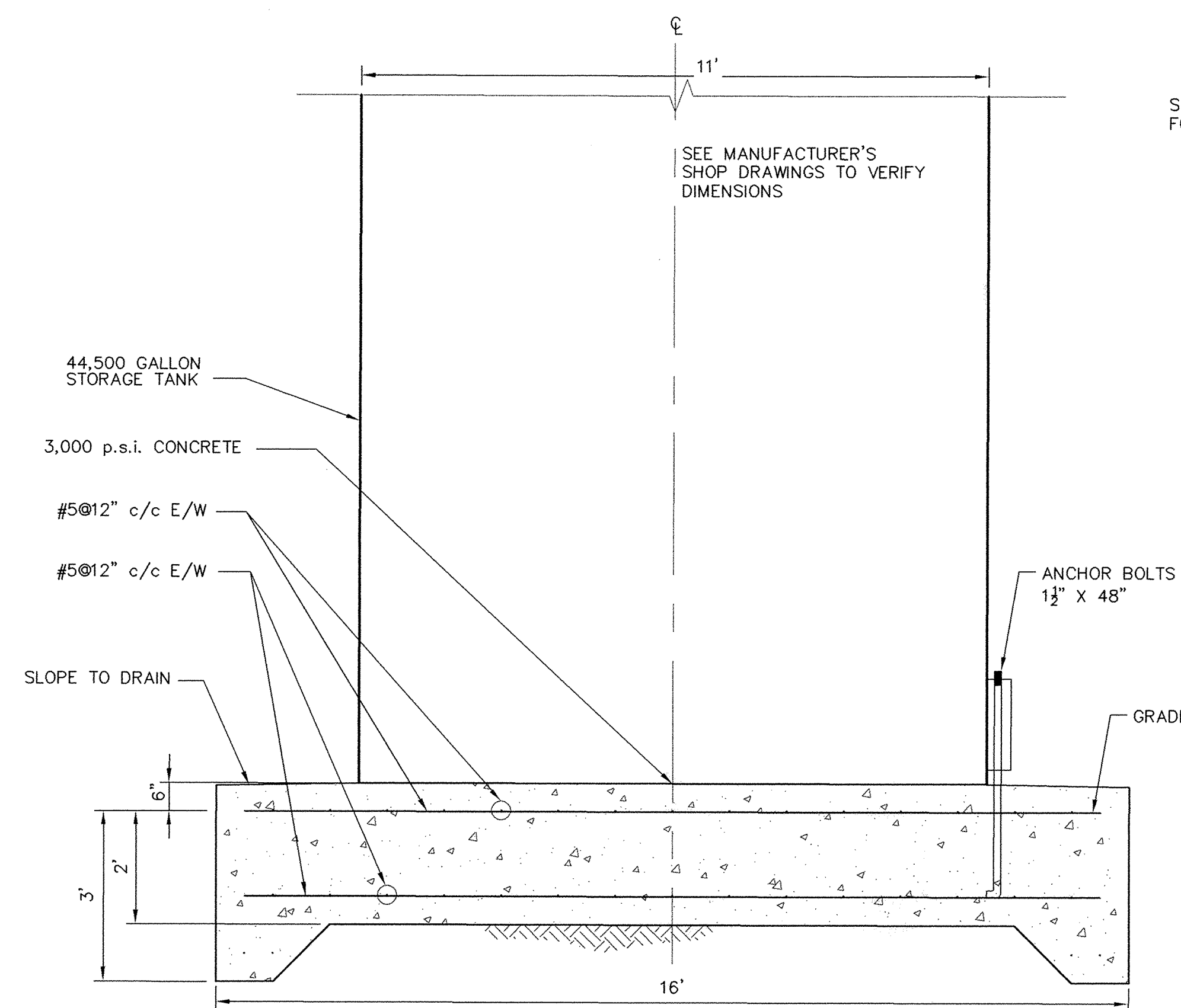
STORAGE TANK FOUNDATION
