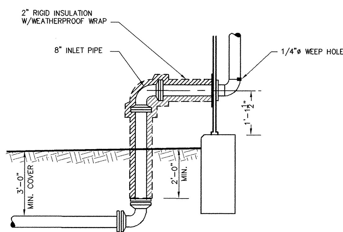
② DETAIL - INLET PIPE NOT TO SCALE
