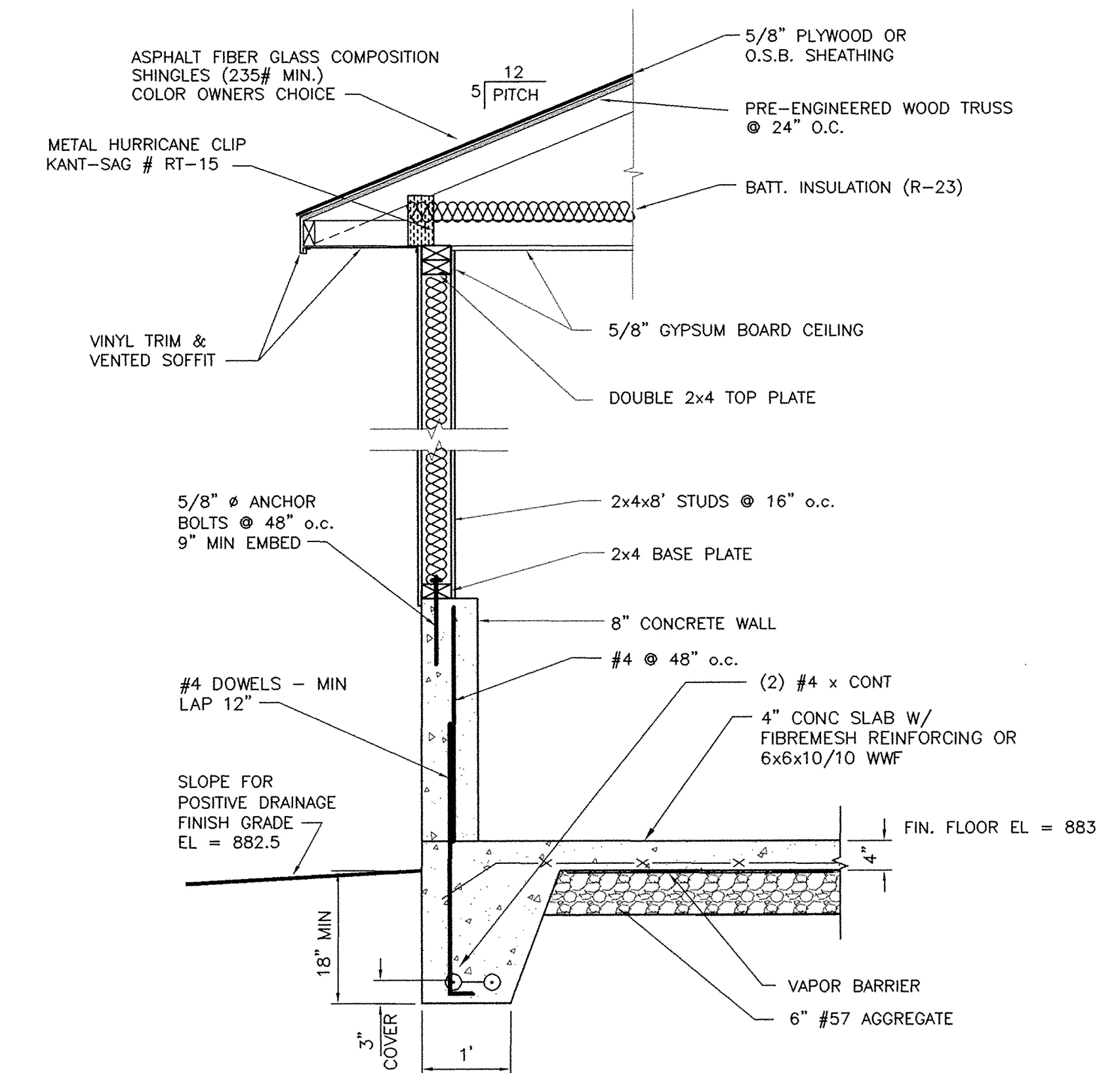
1 TYPICAL WALL SECTION SCALE: 3/4" = 1'-0"
