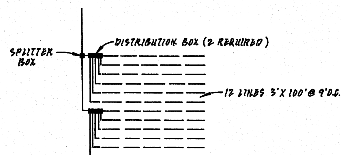
TYPICAL DRAINFIELD LAYOUT DRAINFIELDS 1, 2, 4, 5, 6, 8, 9
