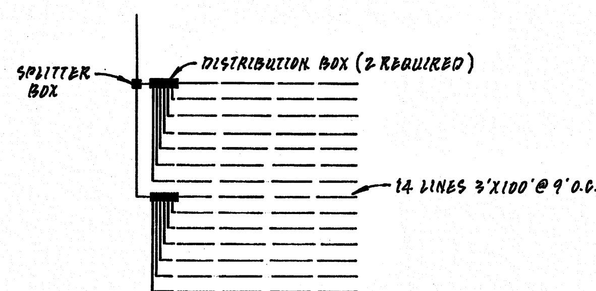
DRAINFIELD 7 LAYOUT
